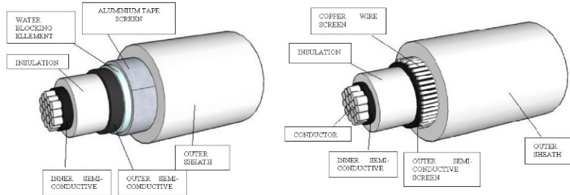
Cable with reduced thickness insulation and Aluminium tape screen.
