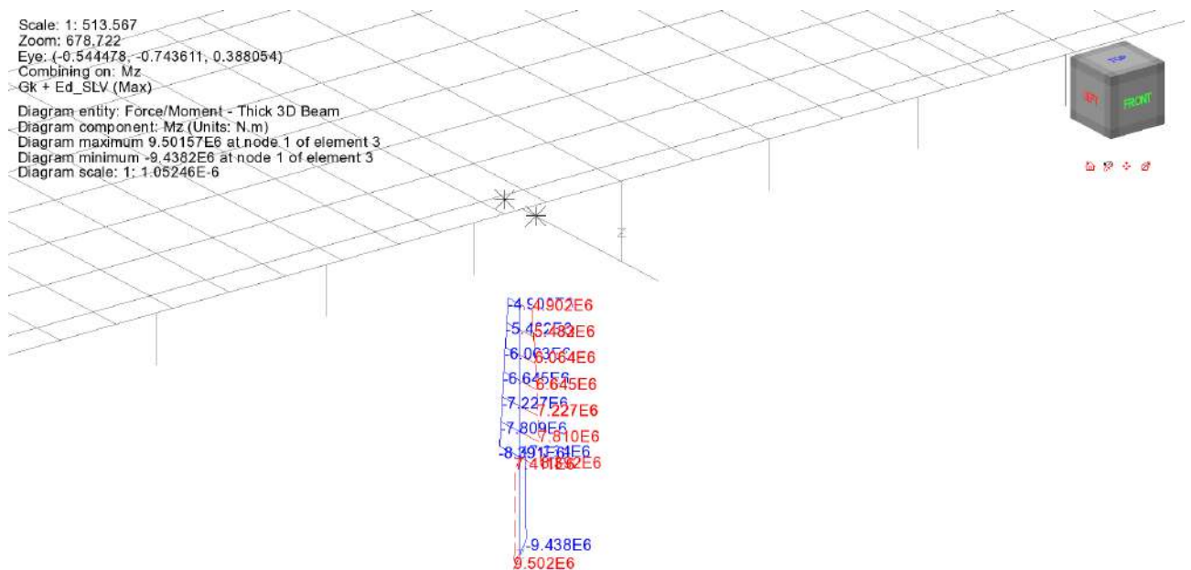
Figura 12.4 My SLV pila - NomDP analysis
