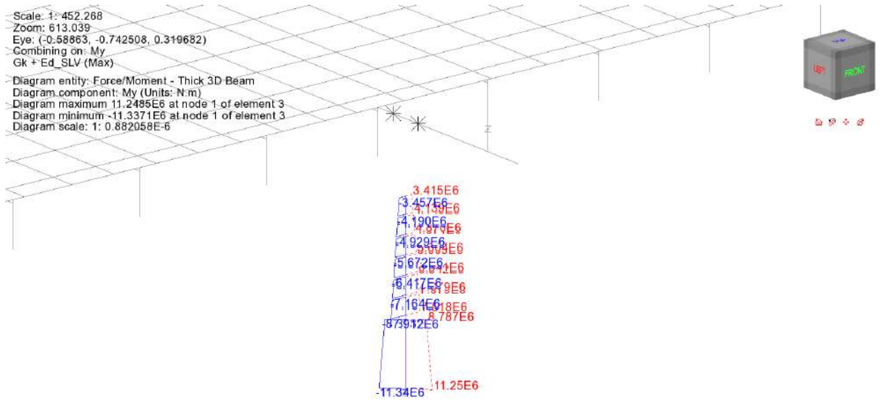
Figura 12.6 My SLV pila - UBDP analysis
