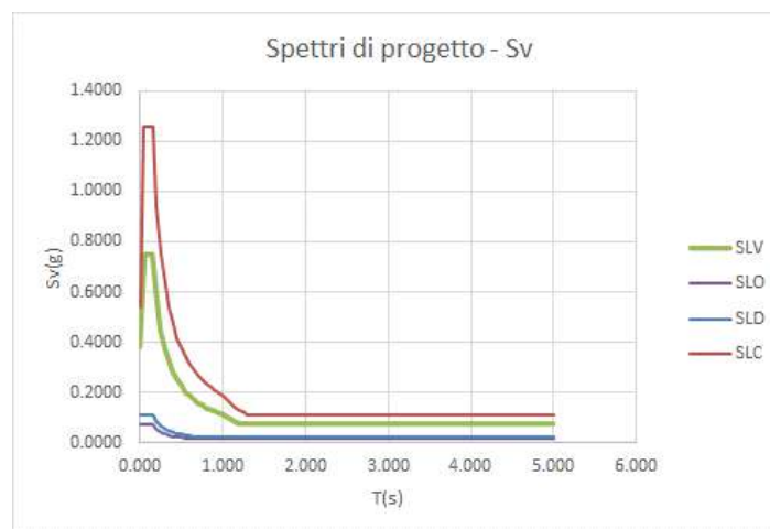
Figura 4.3: Diagramma Sv (g)
