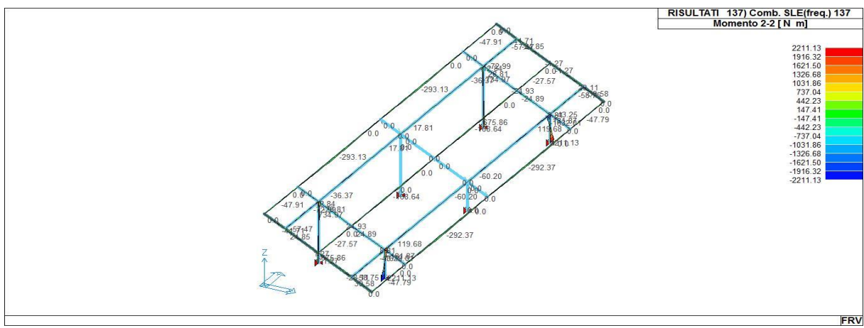
43_RIS_M2_137_Comb. SLE(freq.) 137
