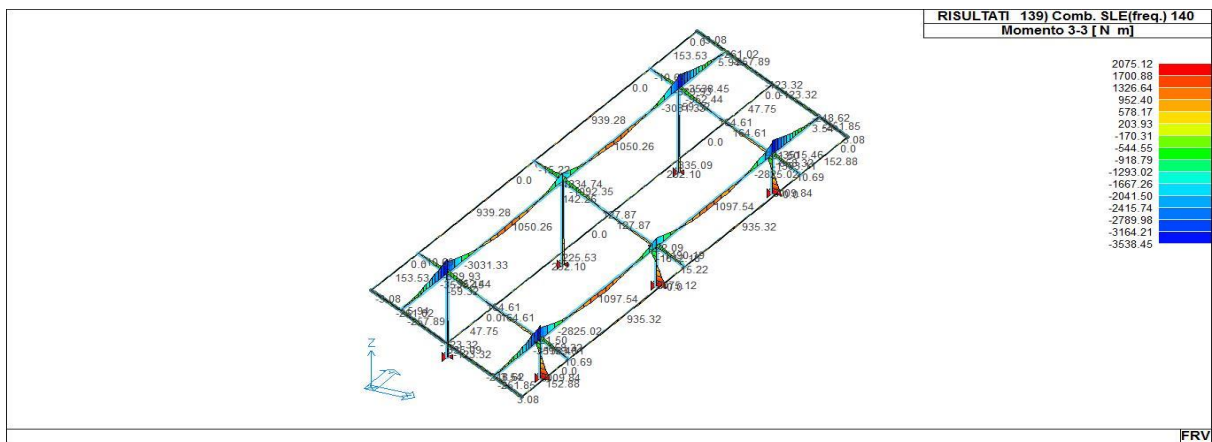
43_RIS_M3_139_Comb. SLE(freq.) 140
