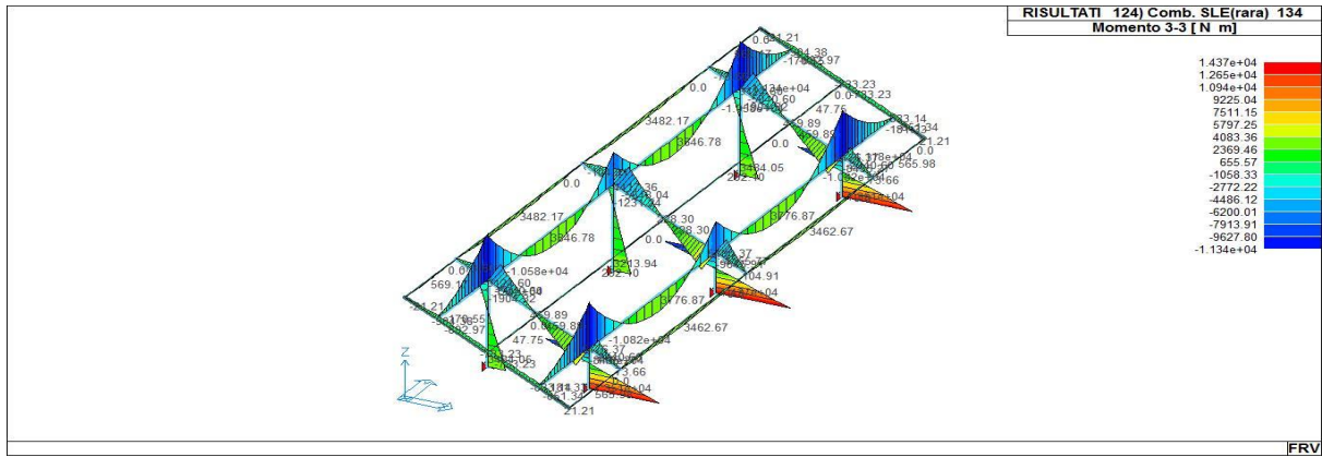
43_RIS_M3_124_Comb. SLE(rara) 134
