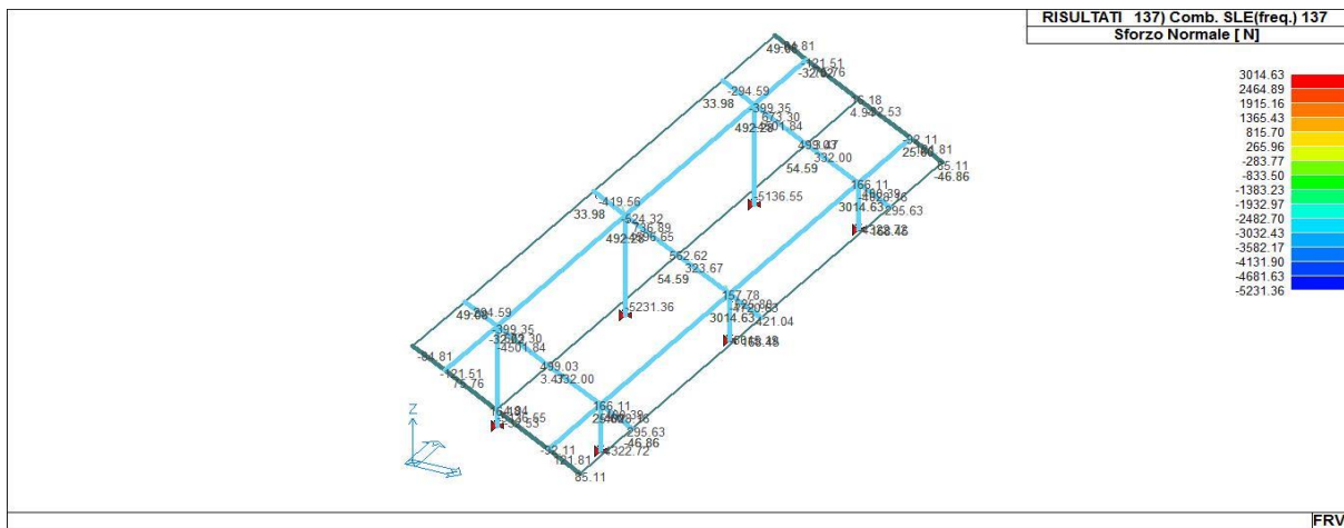
43_RIS_N_137_Comb. SLE(freq.) 137
