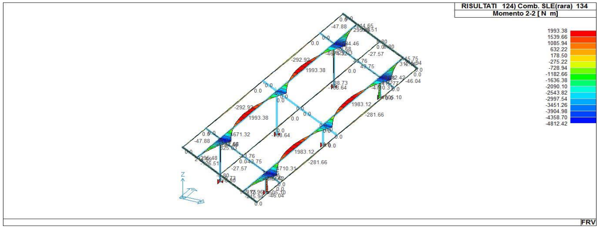
43_RIS_M2_124_Comb. SLE(rara) 134
