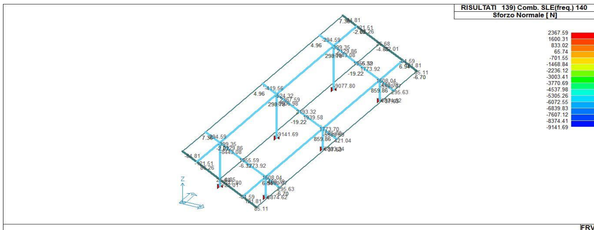
43_RIS_N_139_Comb. SLE(freq.) 140
