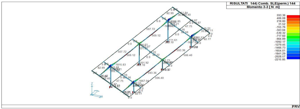
43_RIS_M3_144_Comb. SLE(perm.) 144
