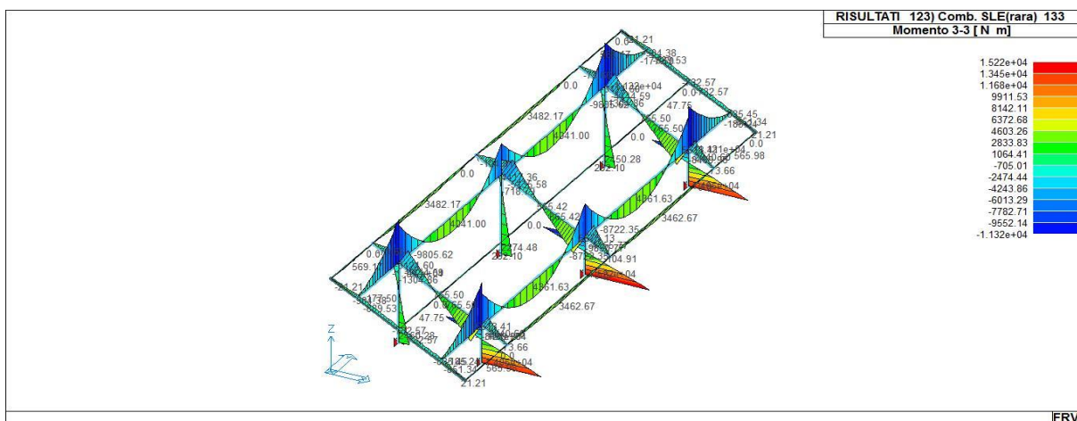
43_RIS_M3_123_Comb. SLE(rara) 133
