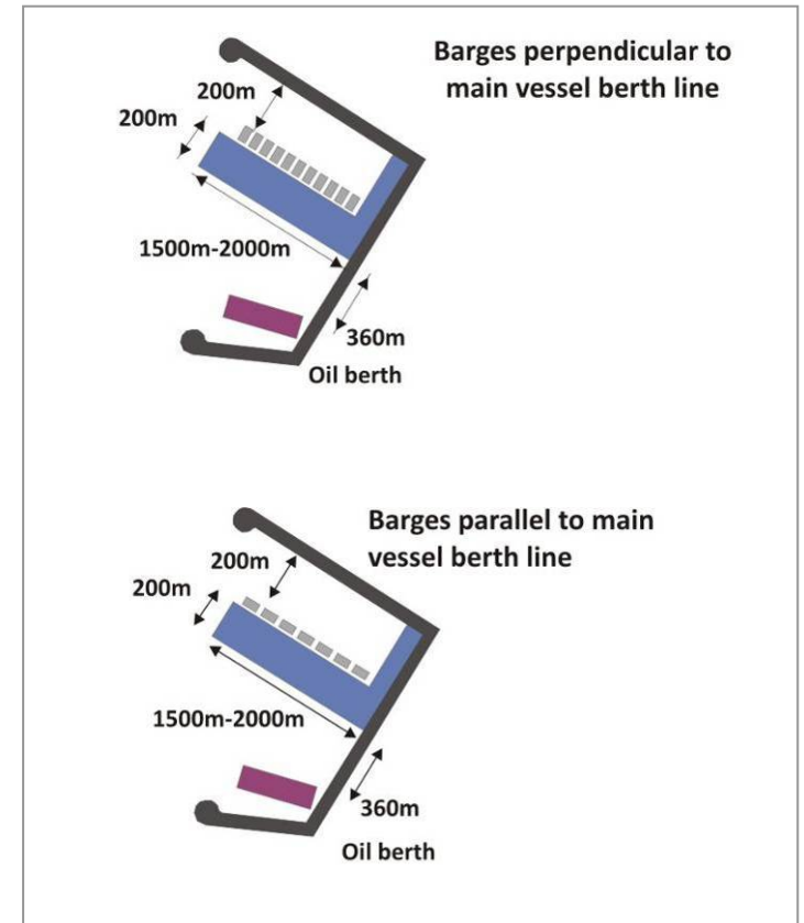
Figure 5-5 Potential concept layouts option 2A
