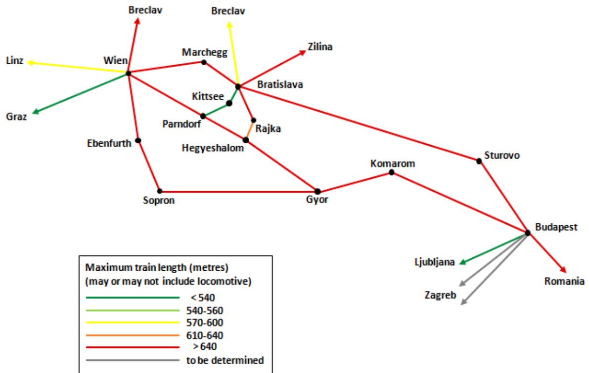
Figure 15: Maximum train lengths in the Wien-Budapest zone
