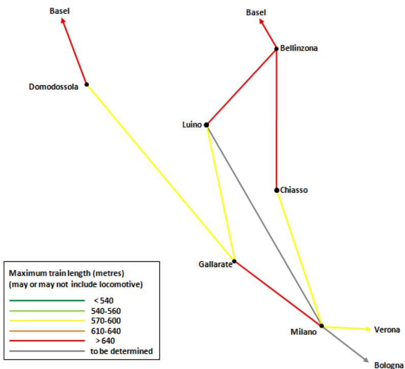
Figure 13: Maximum train lengths in the Milano zone
