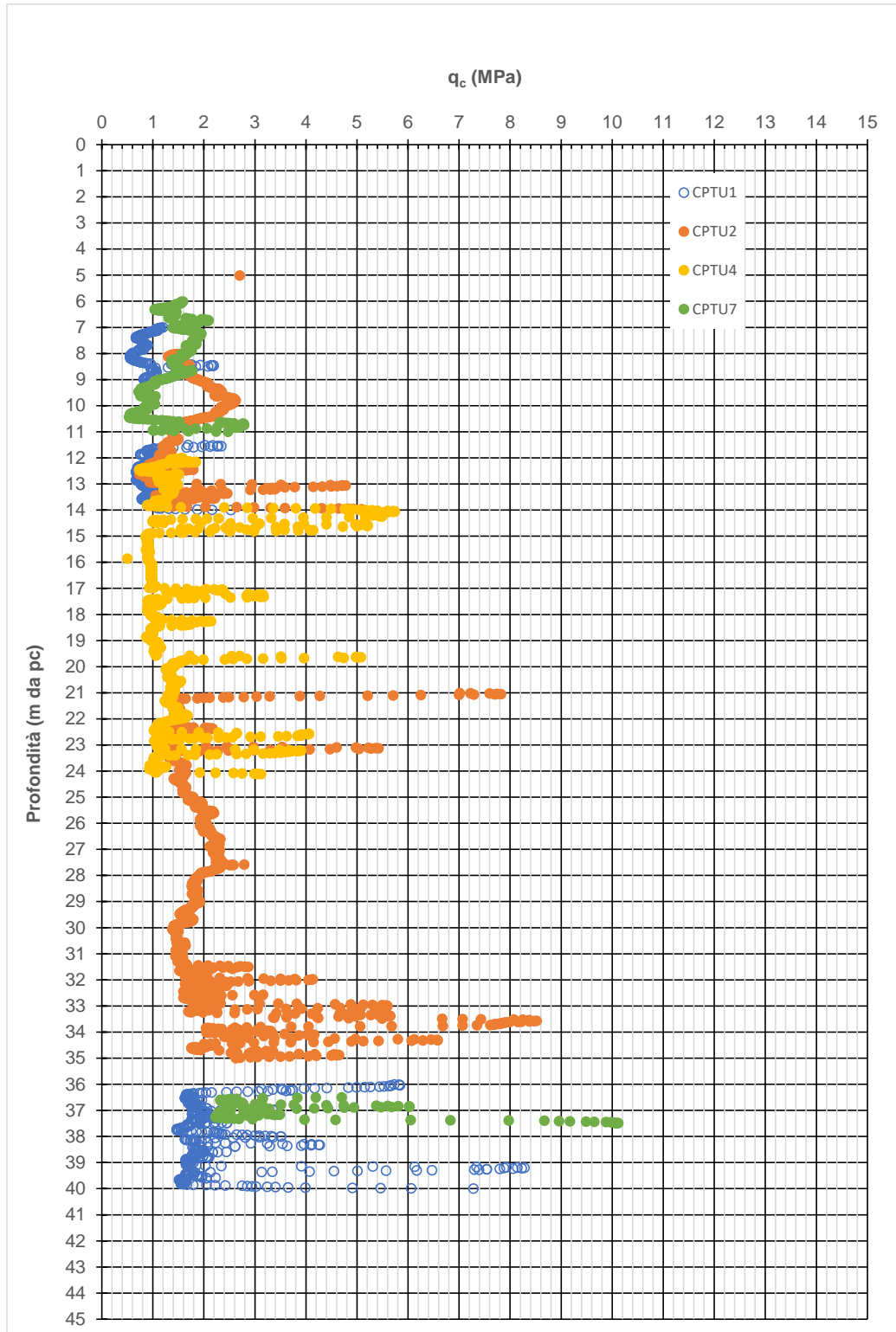
Figura 9-34: AL1 - qc
