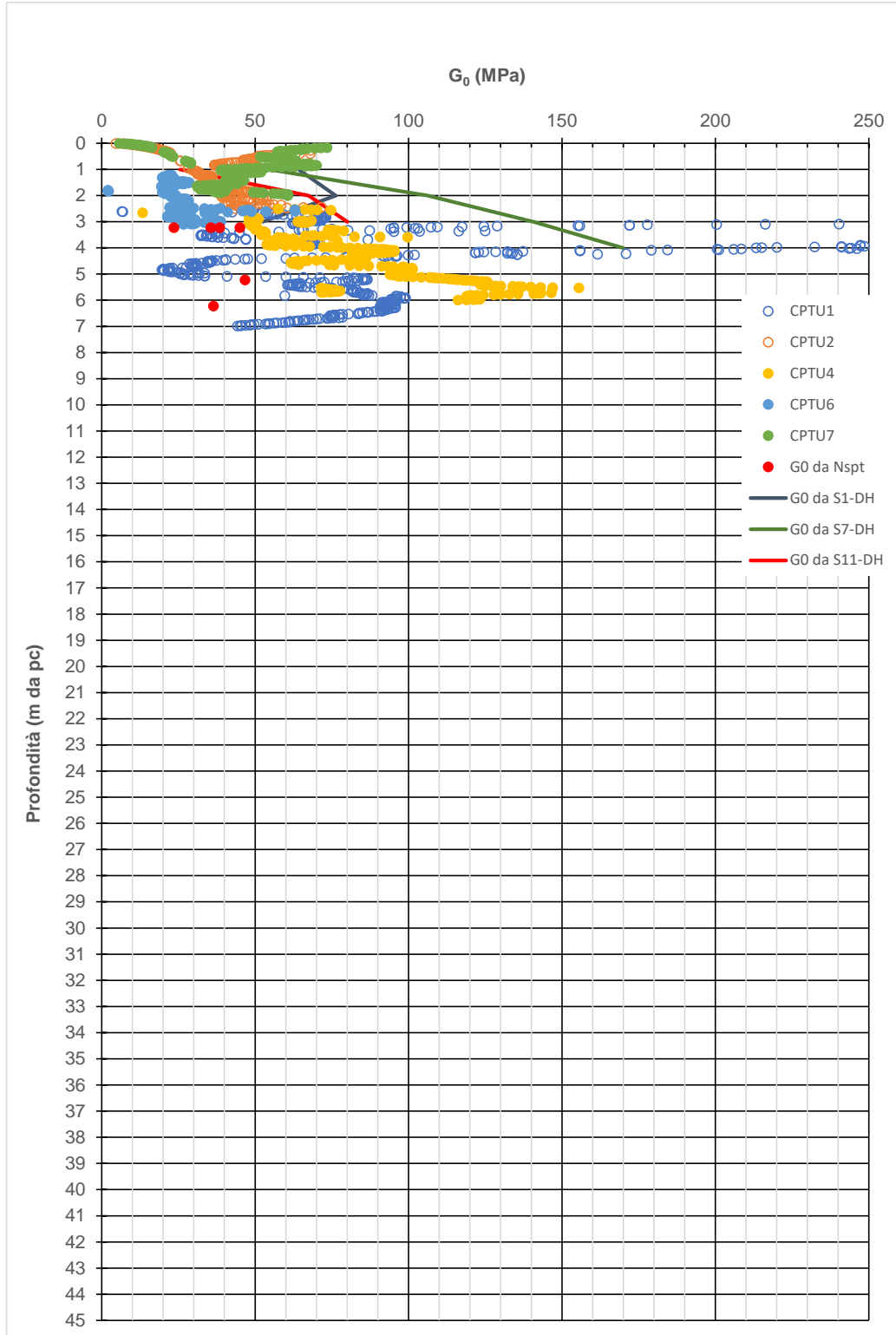
Figura 9-7:R- G_0
