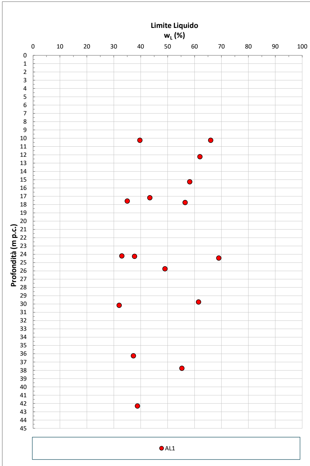
Figura 9-40: AL1 – Limite Liquido
