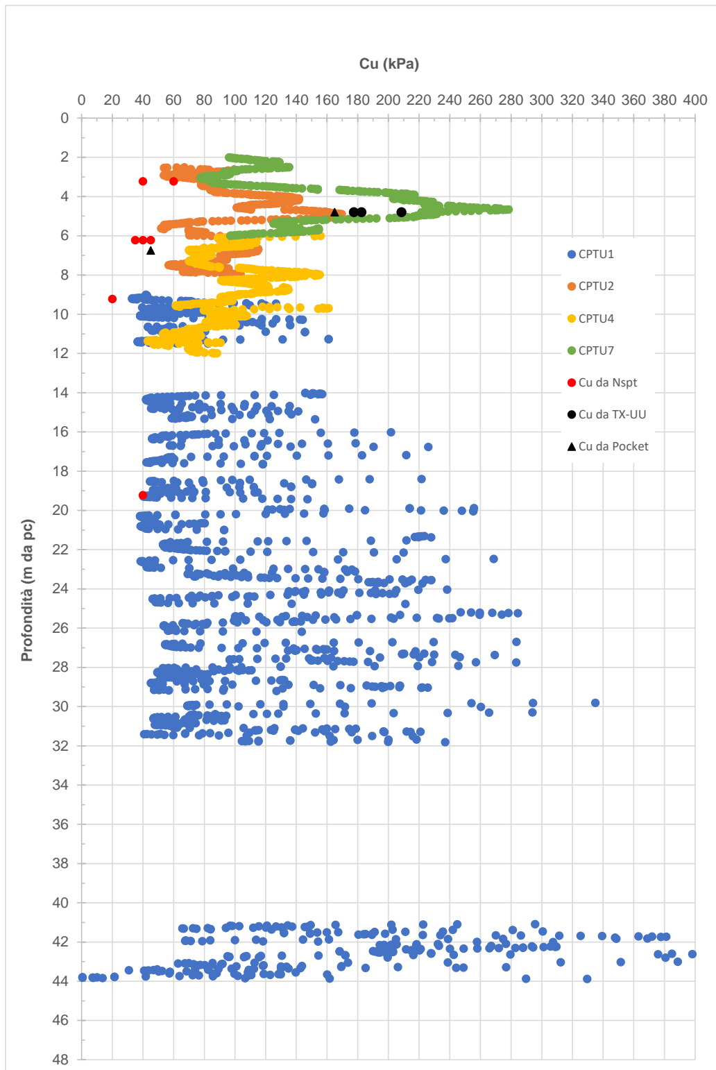
Figura 9-17: LS – c_u
