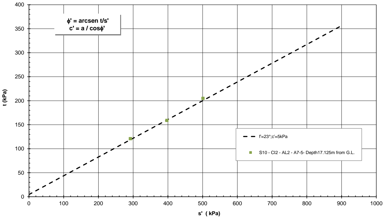
Figura 9-63: AL2 – Prove triassiali TX-CIU
