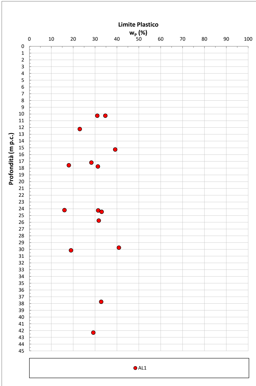
Figura 9-41: AL1 – Limite Plastico
