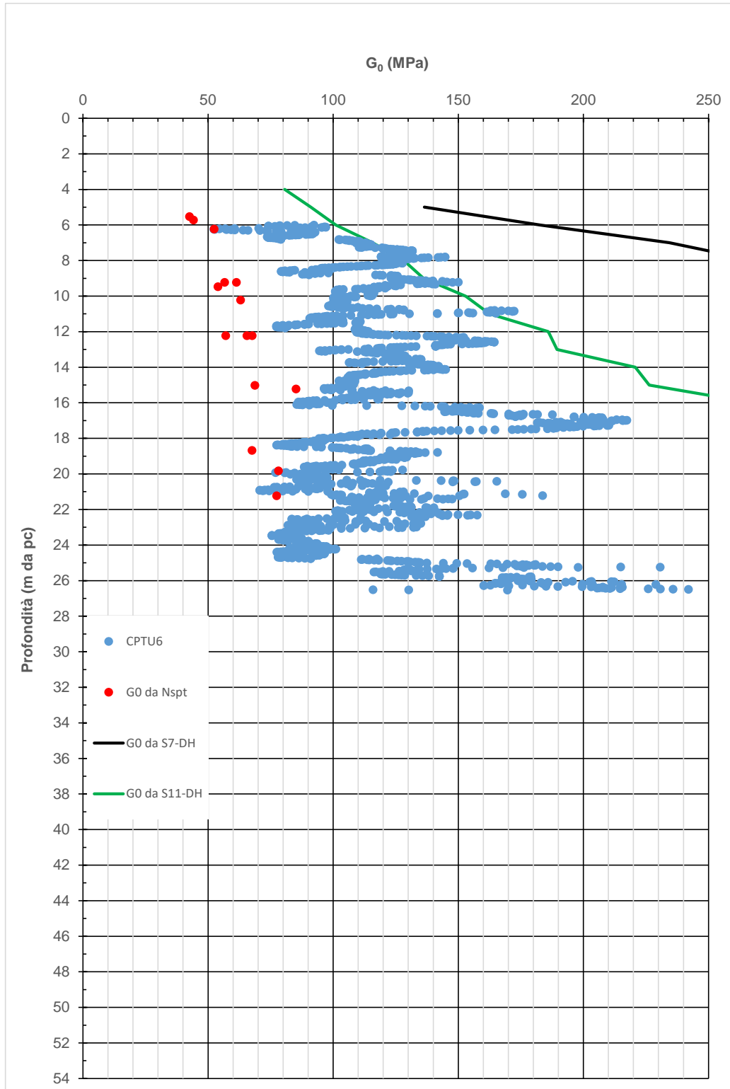
Figura 9-64: AL2 - G_0
