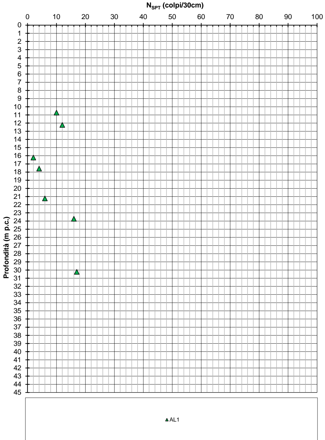
Figura 9-33: AL1 - N SPT
