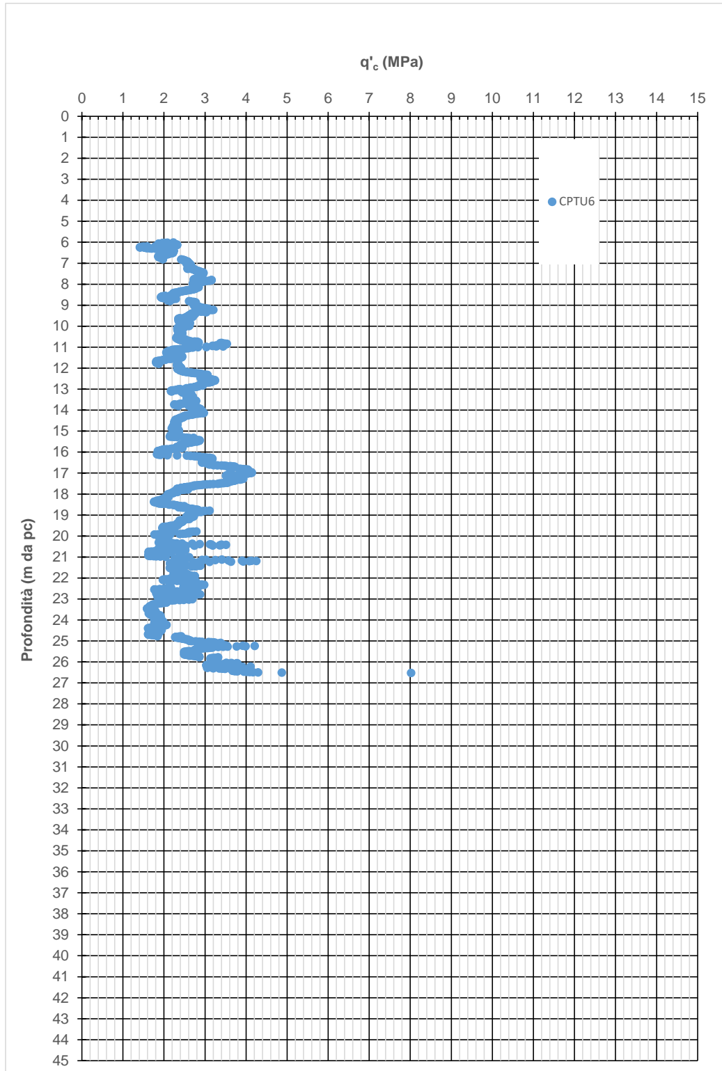
Figura 9-51: AL2 - q_c
