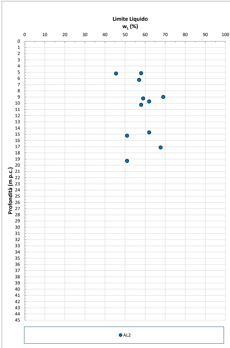
Figura 9-57: AL2 – Limite Liquido
