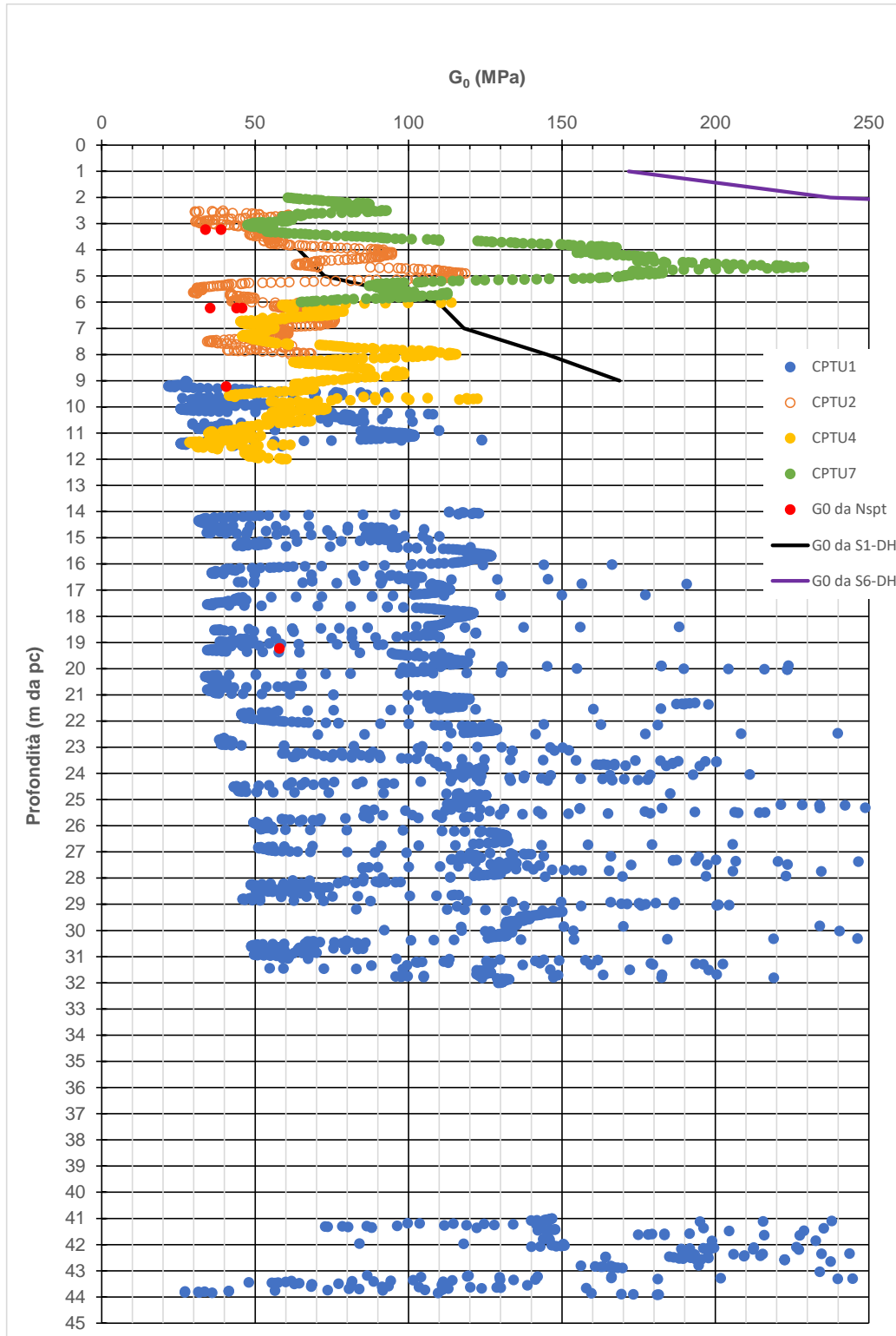
Figura 9-20: LS - G_0
