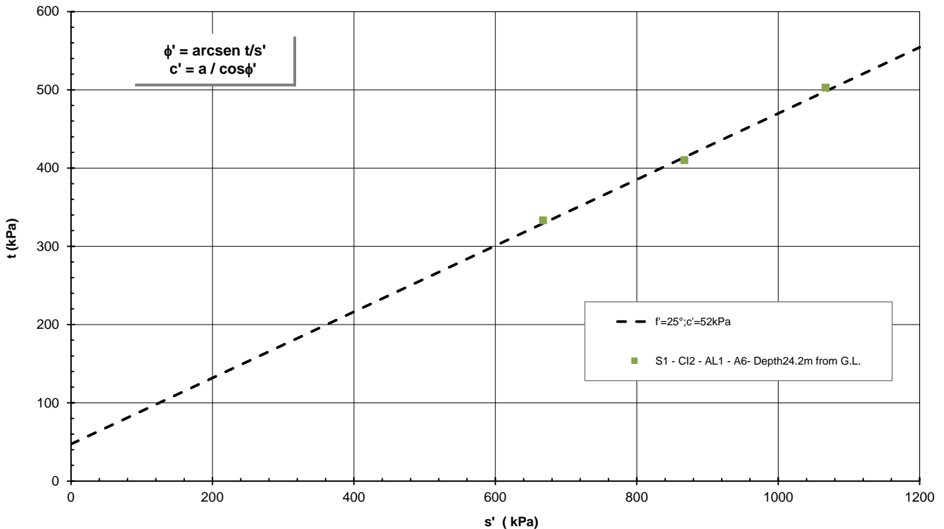
Figura 9-47: AL1 – Prove triassiali TX-CID
