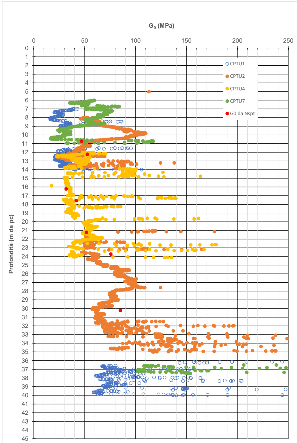
Figura 9-48: AL1 - G_0
