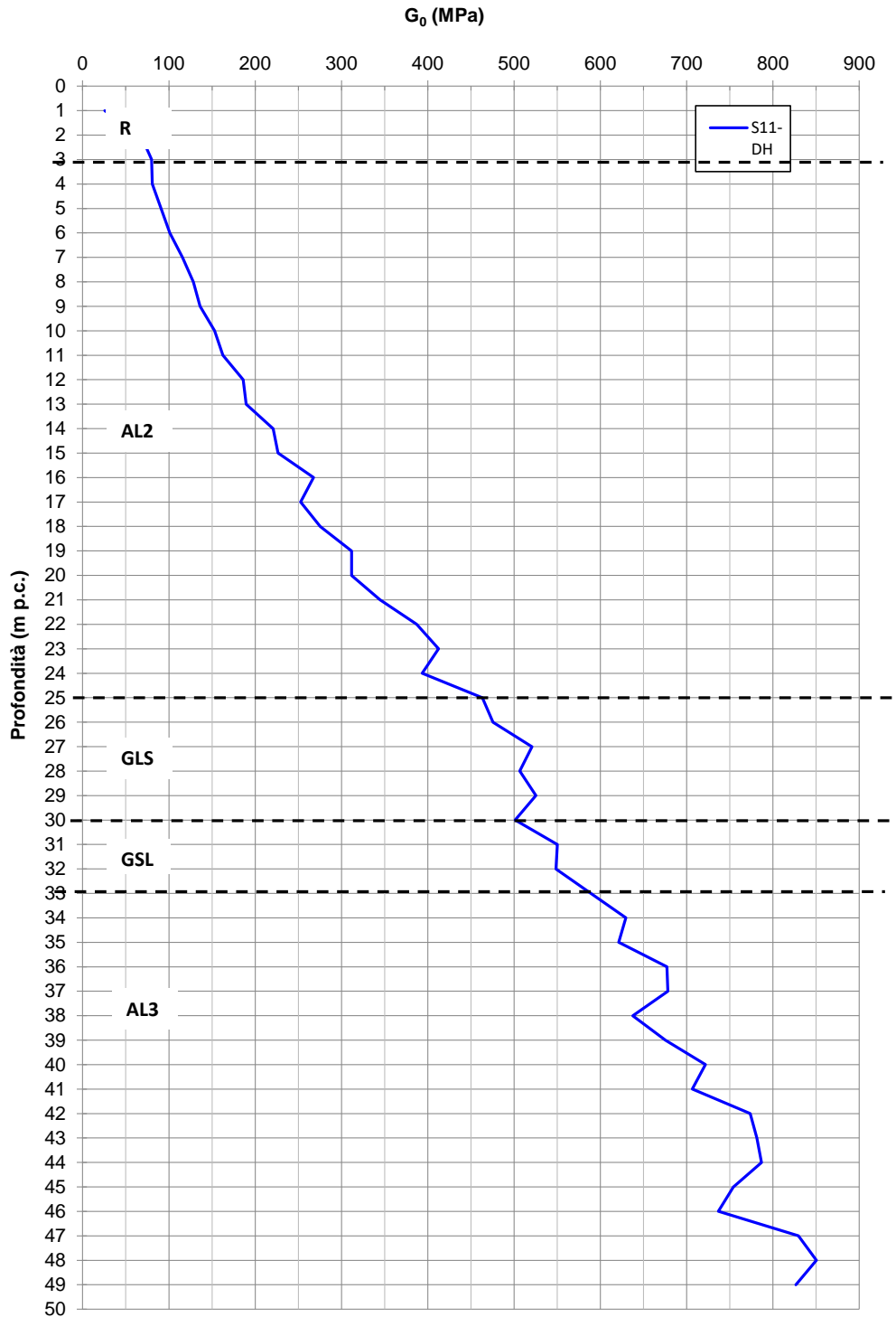
Figura 9-87: AL3 - G_0
