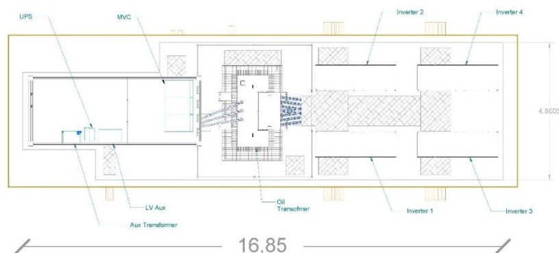
Figura 9: Power station 4 inverters
