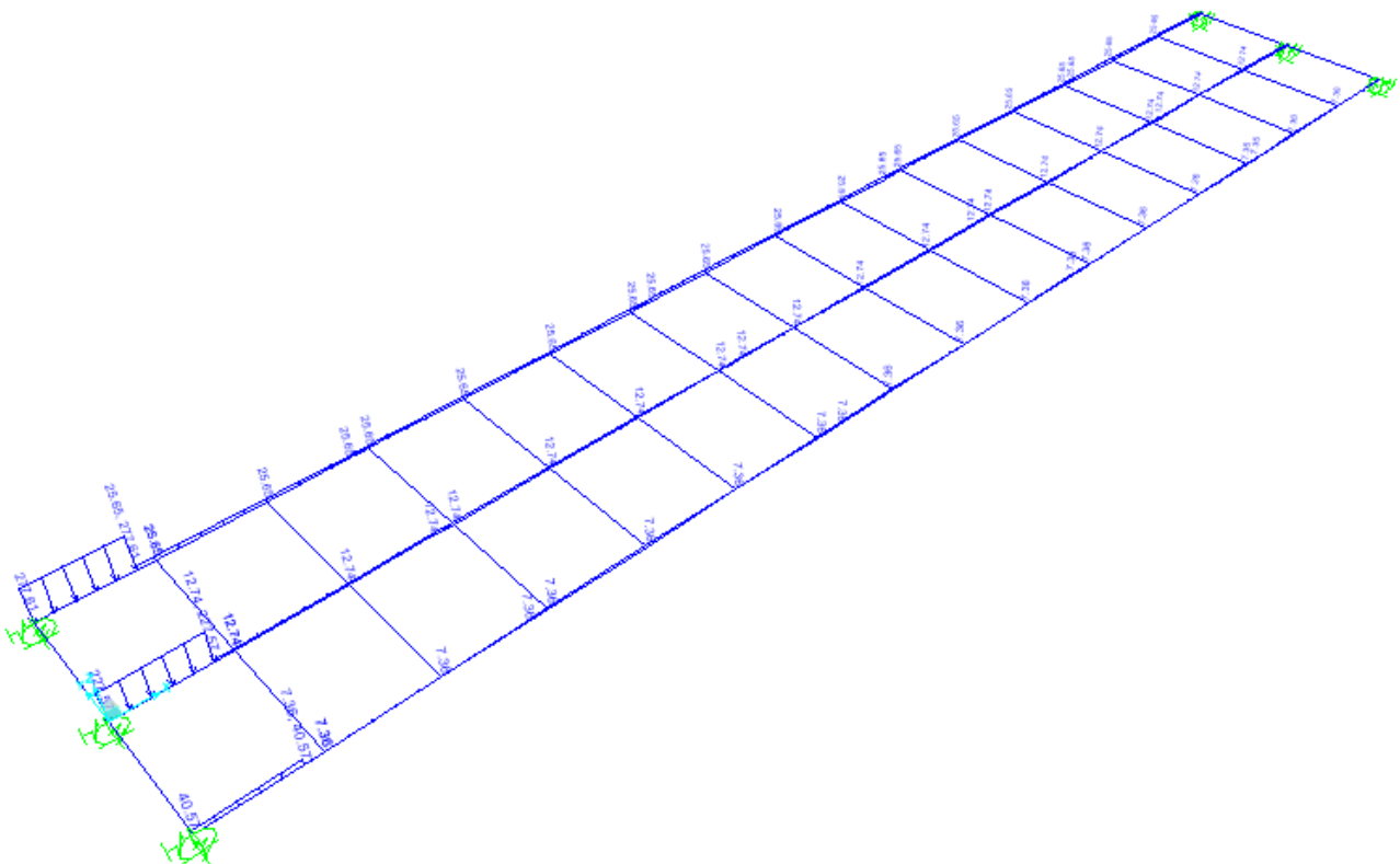
Figura 6.7 Traffico – Mext_M01 01 [kN/m]
