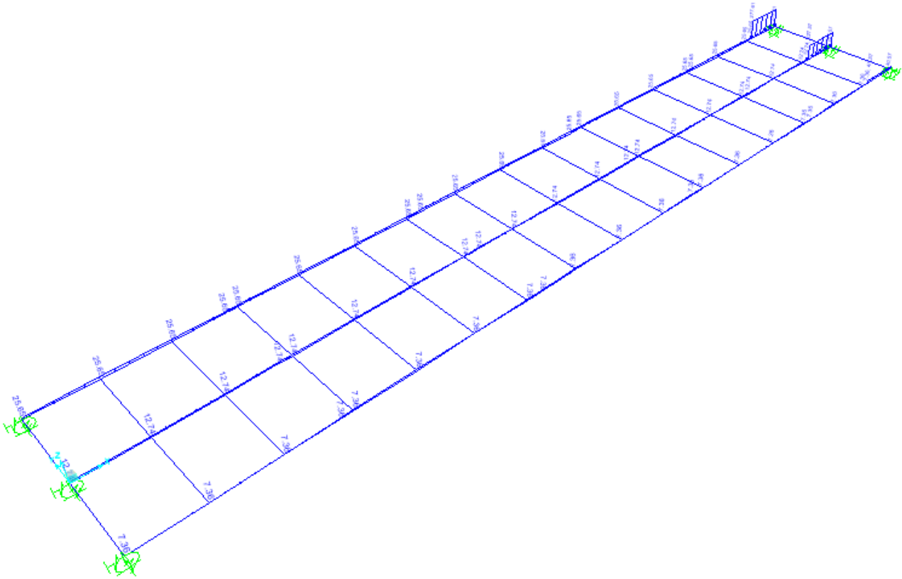
Figura 6.8 Traffico – Mext_M01-31 [kN/m]
