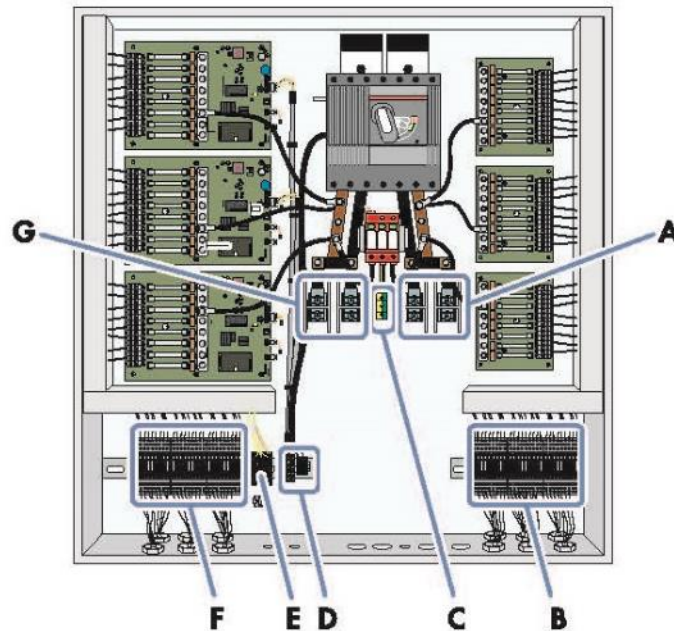
Figure 10: Terminals for connections
