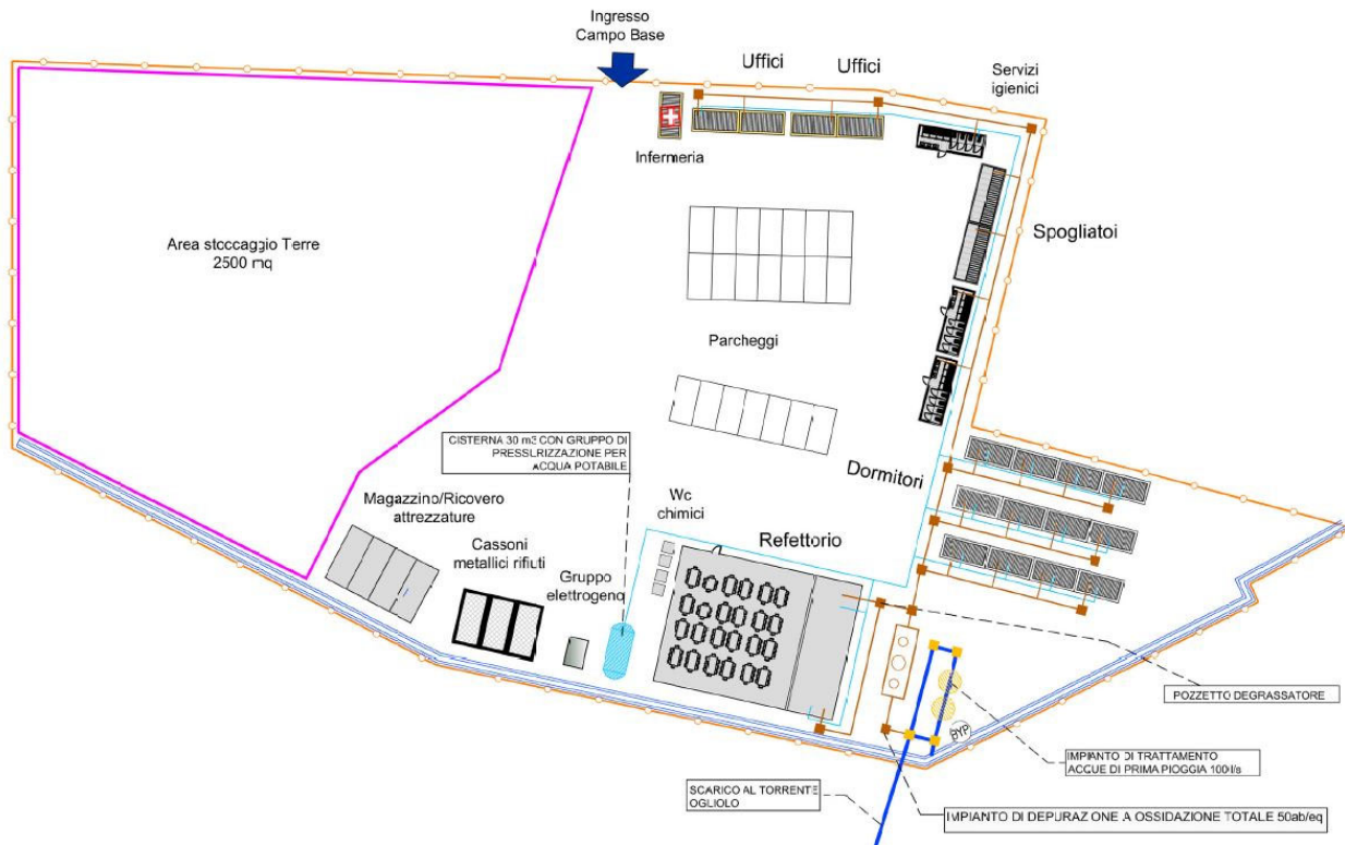
Campo base – Planimetria
