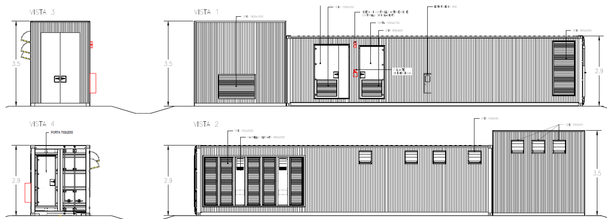
Figura 2.41: Tipologico Power Station
