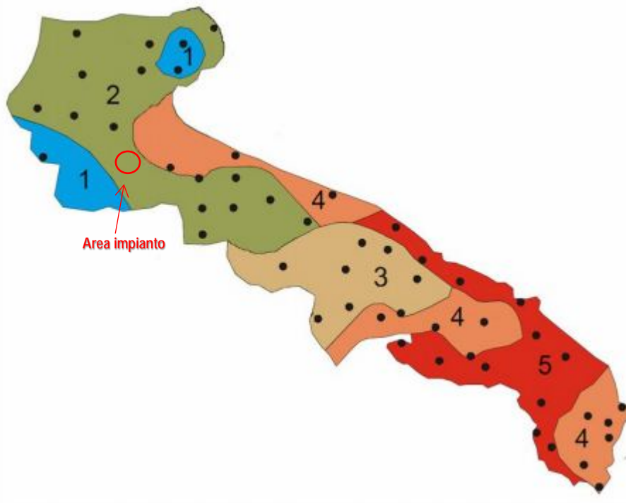
Aree meteo-climatiche
