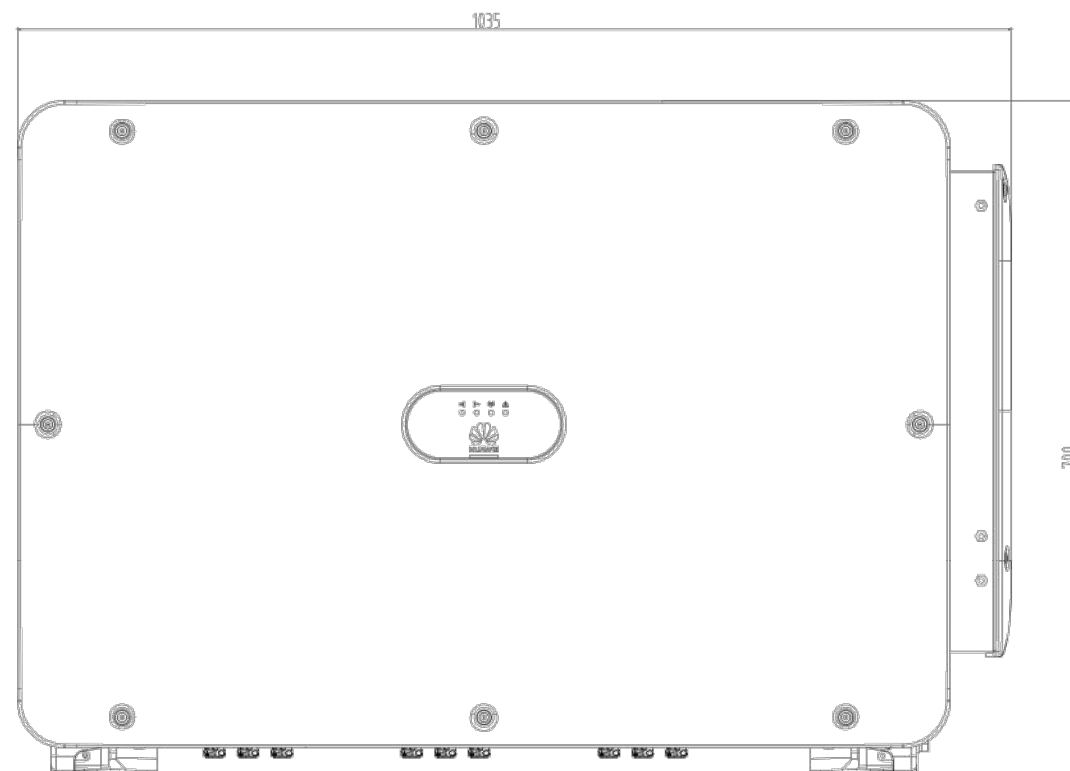
PARTICOLARE INVERTER HUAWEI
