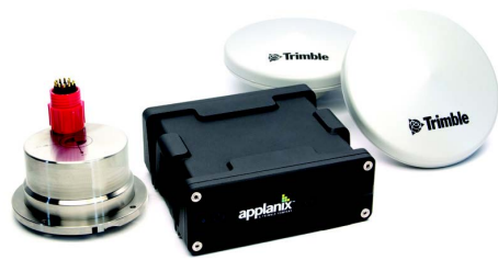
Figura 2.5 Applanix POS-MV
