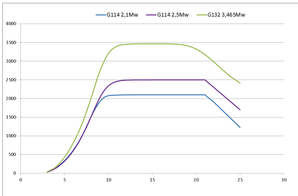
Figure 3.- Siemens-Gamesa G132 3.465 MW power curve
