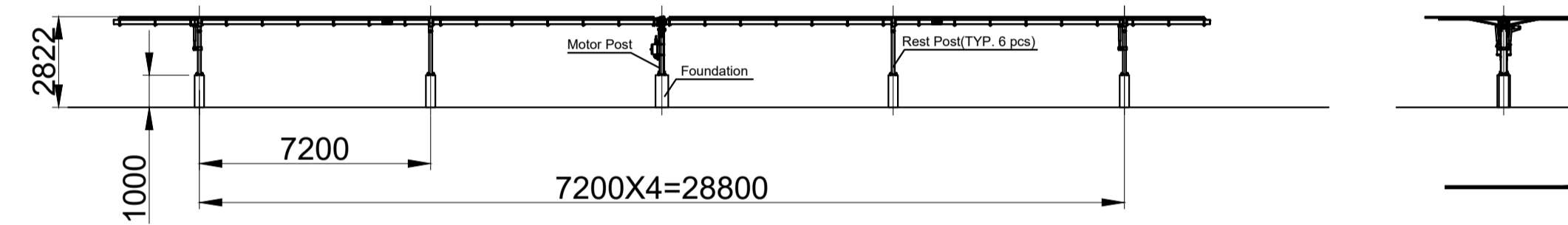
1 row, each row has 60 modules
