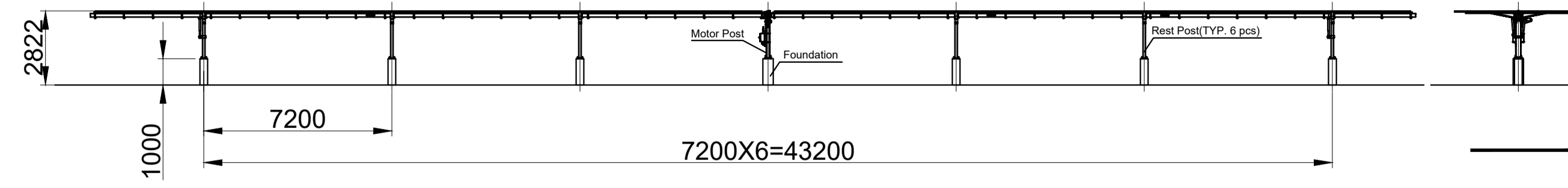
1 row, each row has 90 modules
