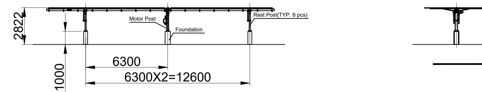
1 row, each row has 30 modules
