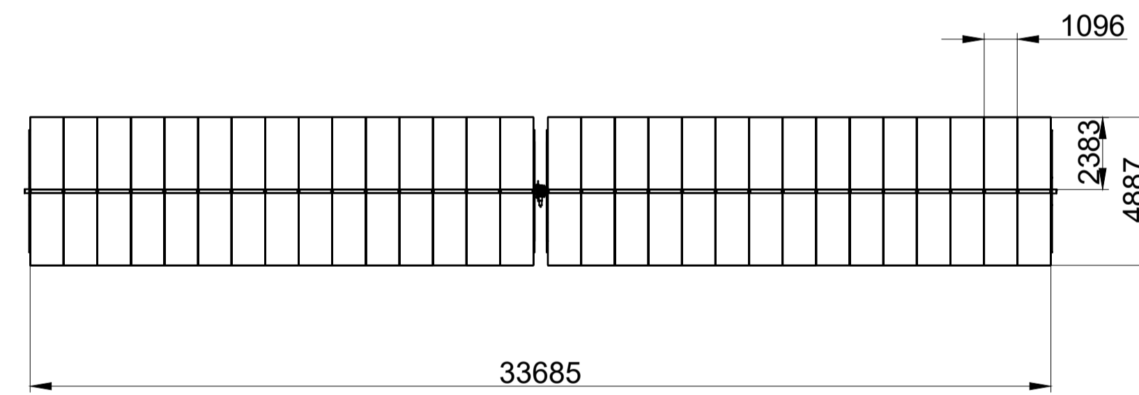
1 row, each row has 60 modules
