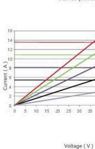
Current-Voltage & Power-Voltage Curves (565W)
