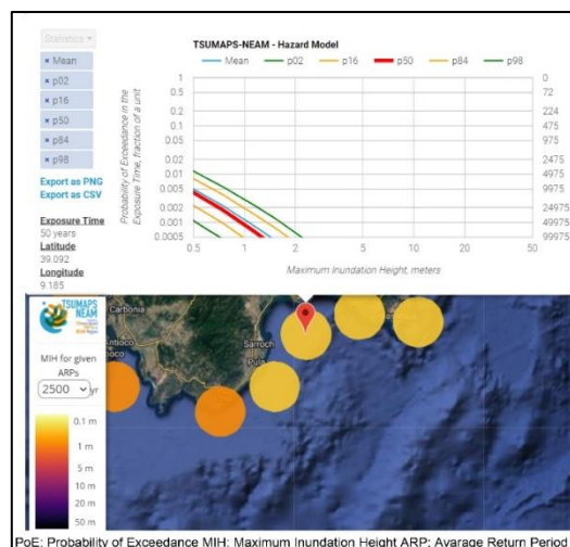
Figura 3.5: NEAM Probabilistic Tsunami Hazard Model 2018 (Refs.[19] & [20])
