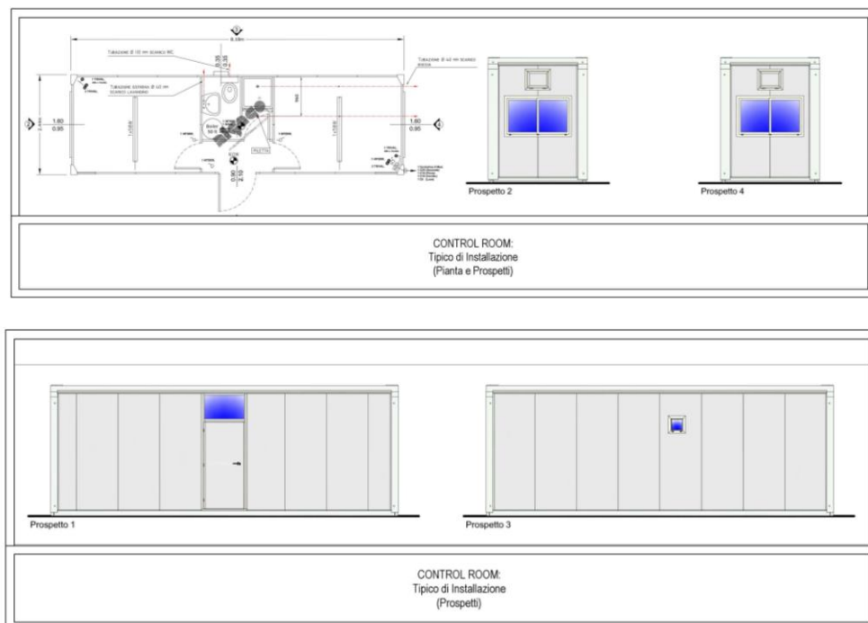
Figura 3.8: Control Room
