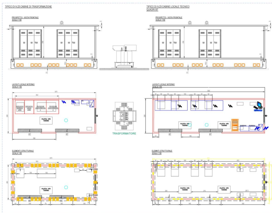
Figura 3.7: Power Station
