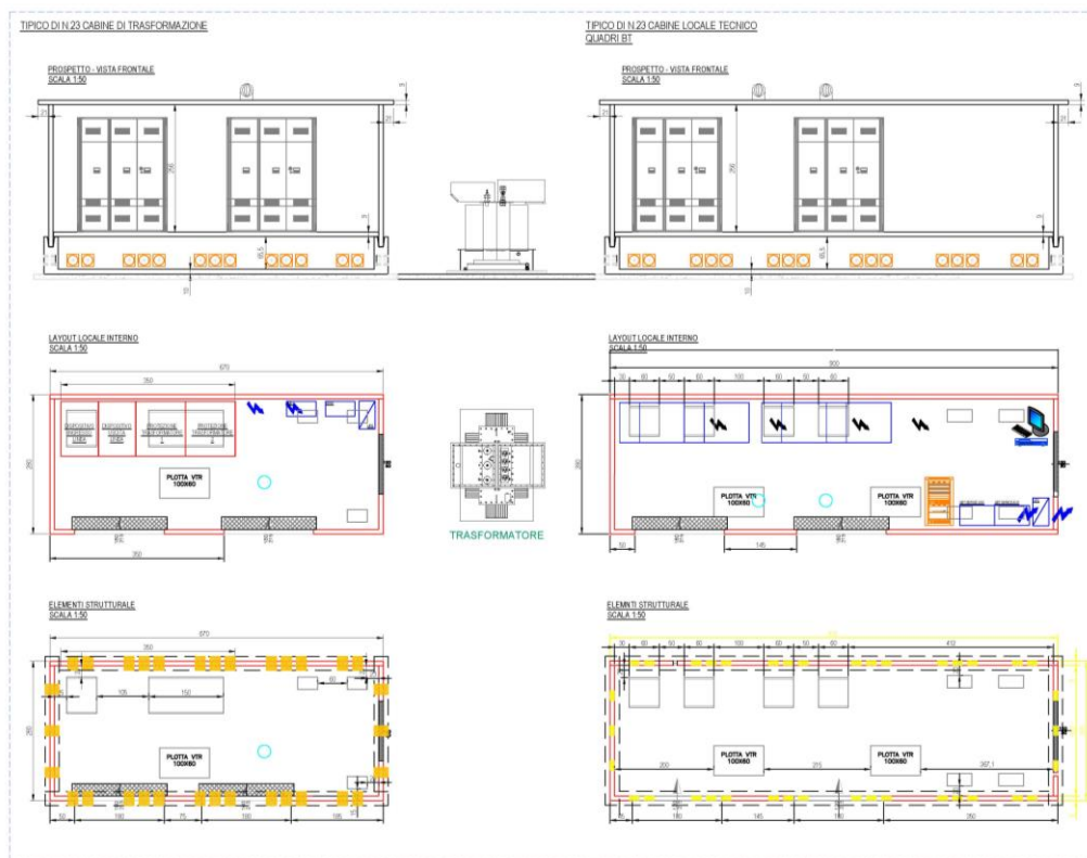
Figura 3.7: Power Station
