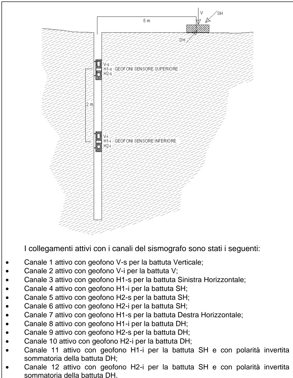
Figura 20 - Down-Hole_Schema operativo
