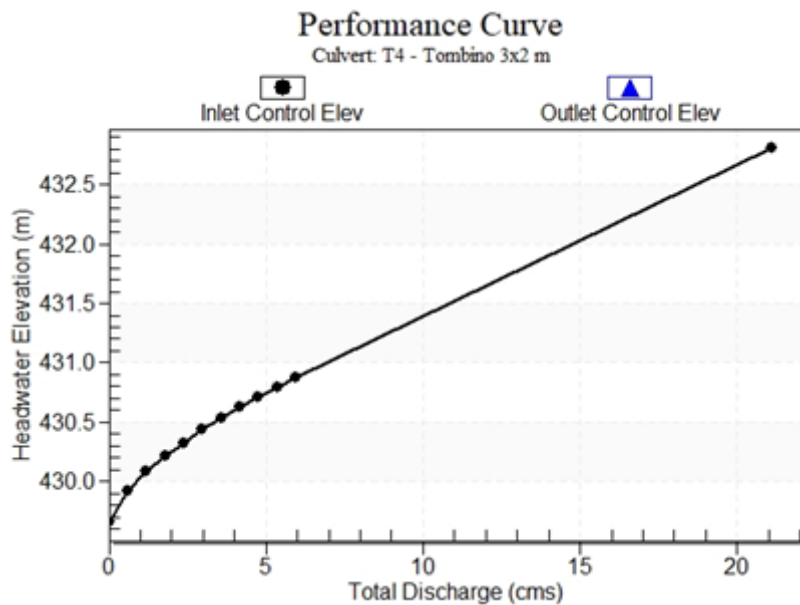
Figura 125 - Culvert Performance Curve Plot: T4 - Tombino 3x2 m
