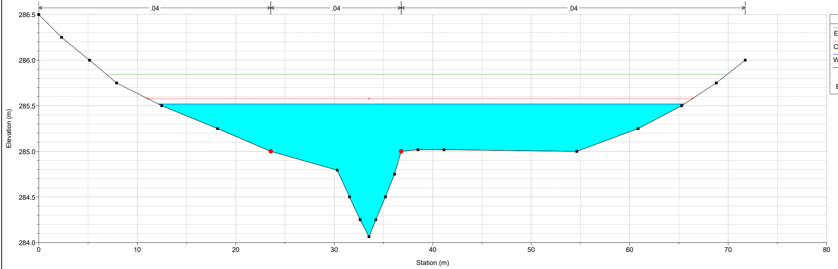
Rio_Mannu Plan: TR200_PRO ver manufatti sez nok 13/05/2020 Sez 4
