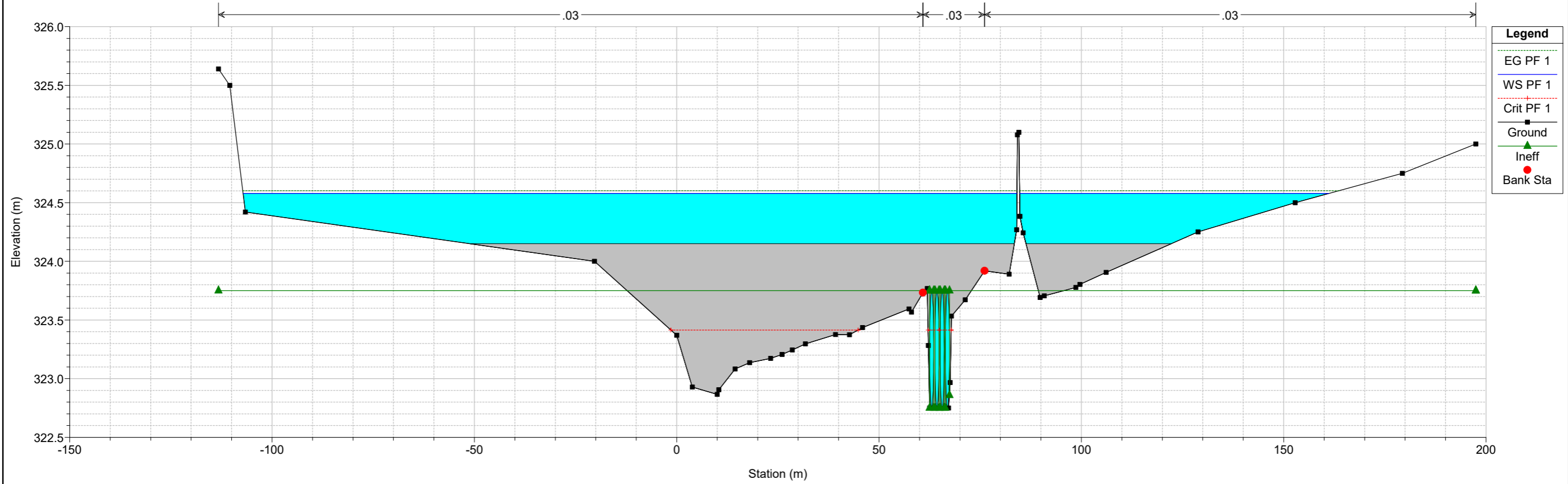
Rio_Bonorchis Plan: Q 200 sdf coeff + ineff + sez all 22/04/2020 Parallela S.S. 131 valle
