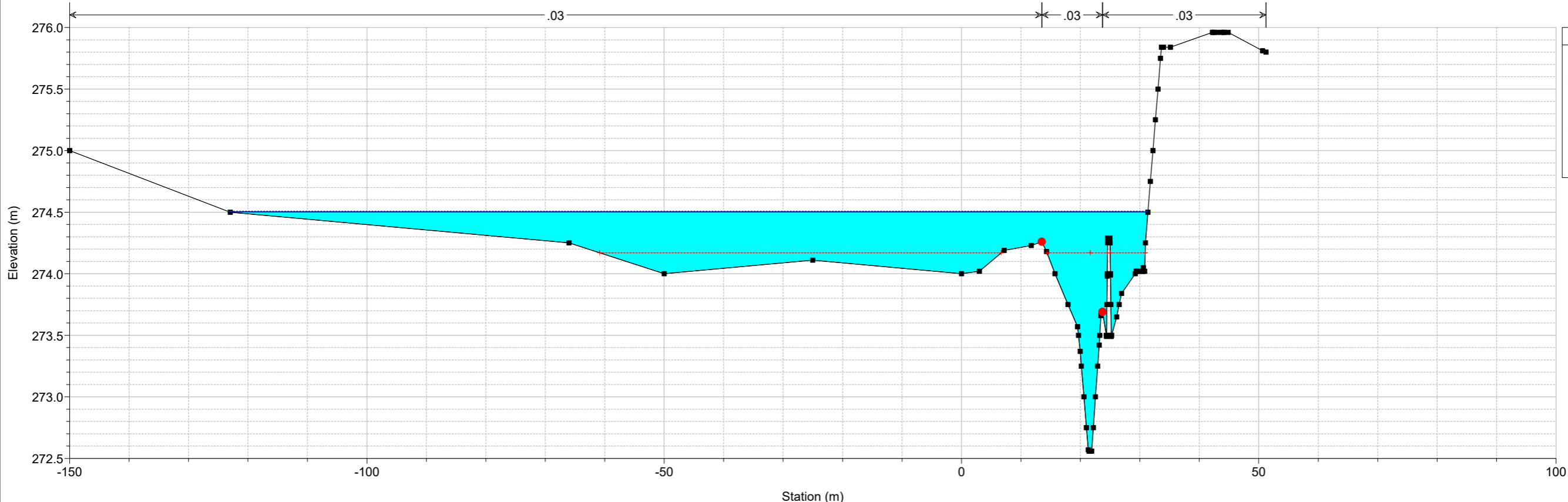
HEC-RAS model from Autodesk® River and Flood Analysis Module 2020 Plan: Tr200 sdf mod sez 22/05/2020 Sez. 14
