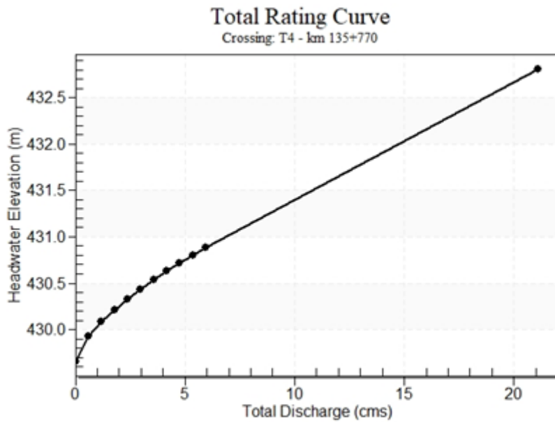
Figura 124 - Rating Curve Plot for Crossing: T4 - km 135+770
