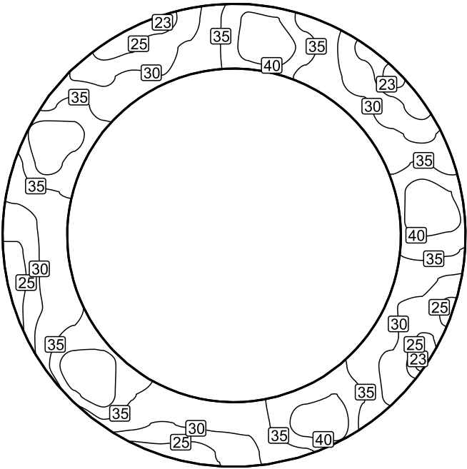
Isolinee [lx]
