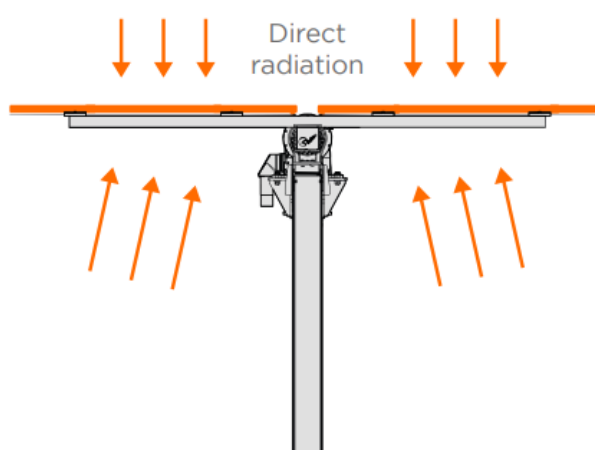
Figura 7: Back Tracking
