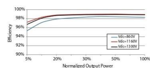
EFFICIENCY CURVE
