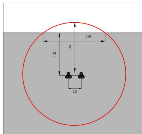
Cavo ARG7H1E(X) 18/30 kV 300 mm 2
