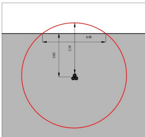
Cavi ARG7H1E(X) 18/30 kV 185 mm 2
