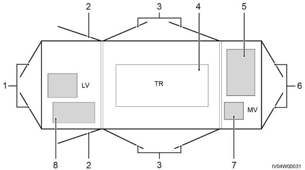
Figure 2-3 Layout
