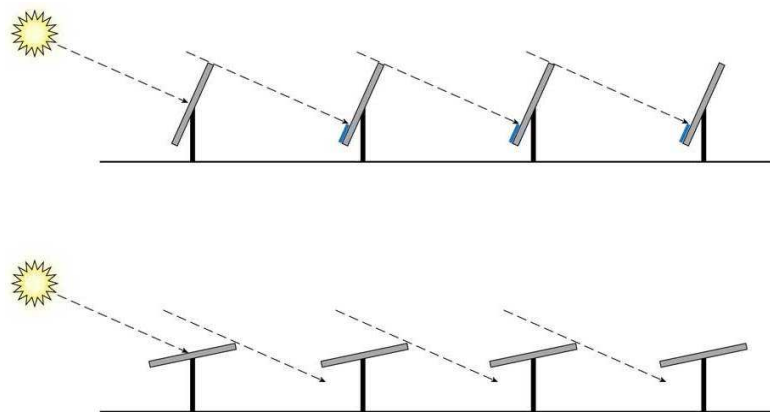
Figure 1: Backtracking
