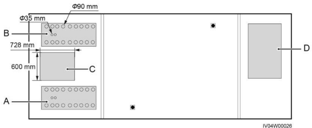
Figure 2-8 Bottom view
