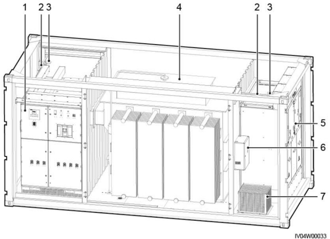
Figure 2-5 Interior
