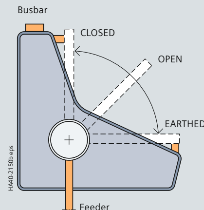
Three-position switch-disconnector
