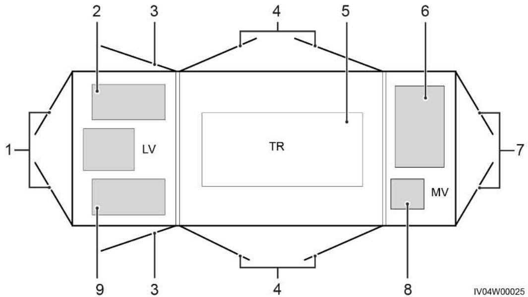
Figure 2-7 Layout
