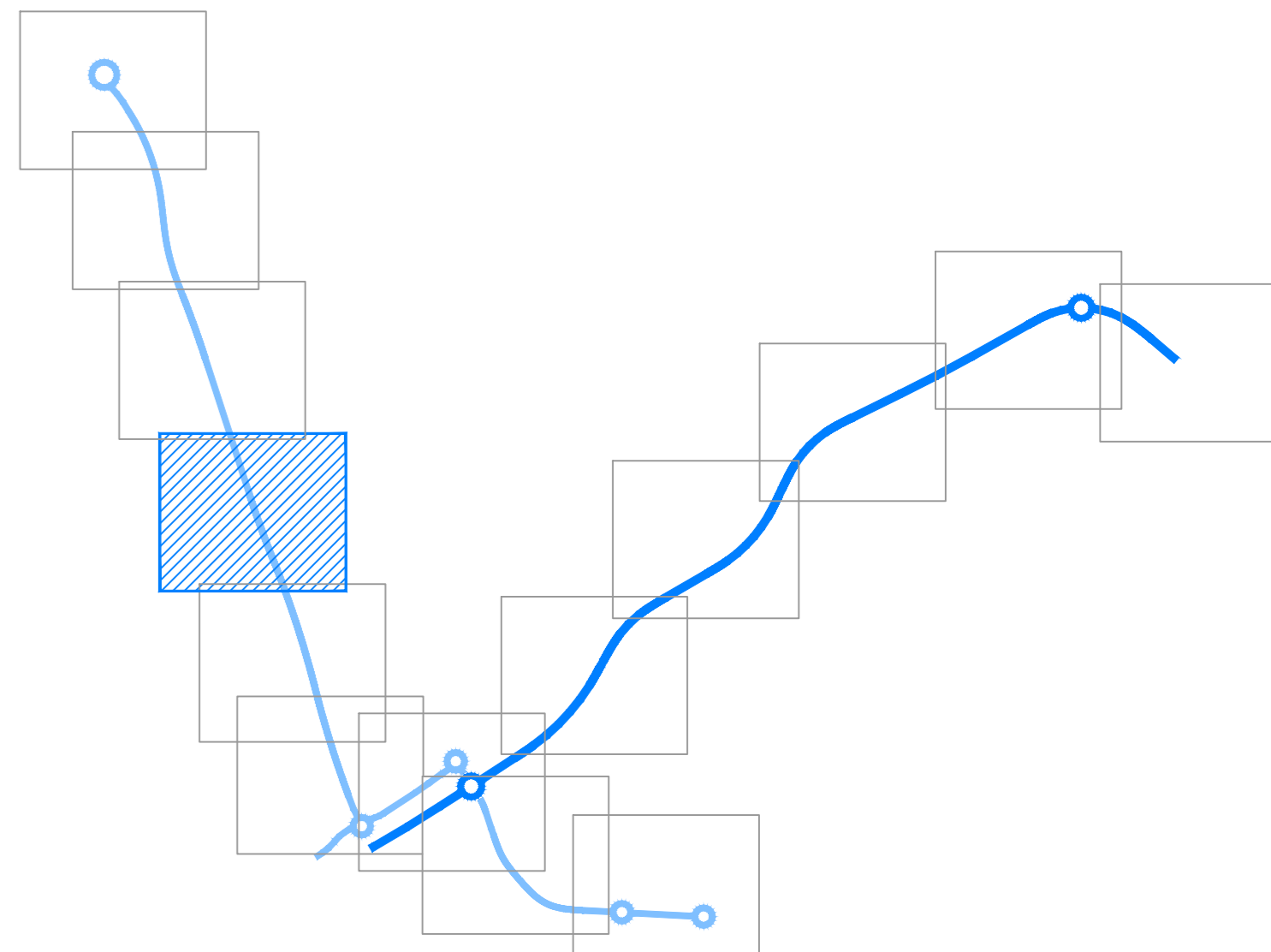
key-map
