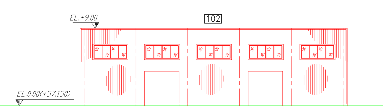
VISTA "A" SCALE 1:250
