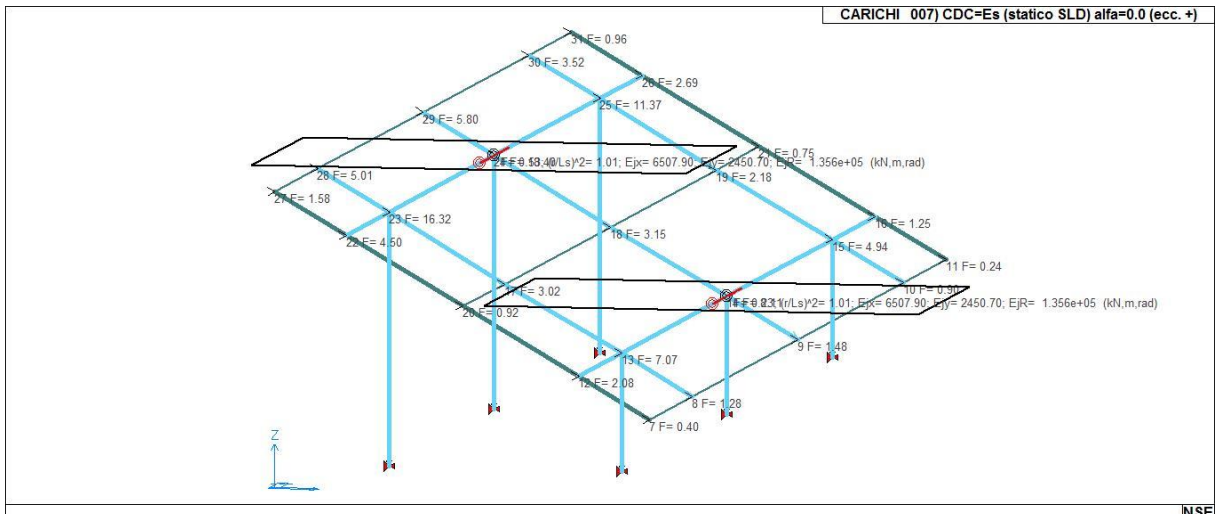
22_CDC_007_CDC=Es (statico SLD) alfa=0.0 (ecc. +)
