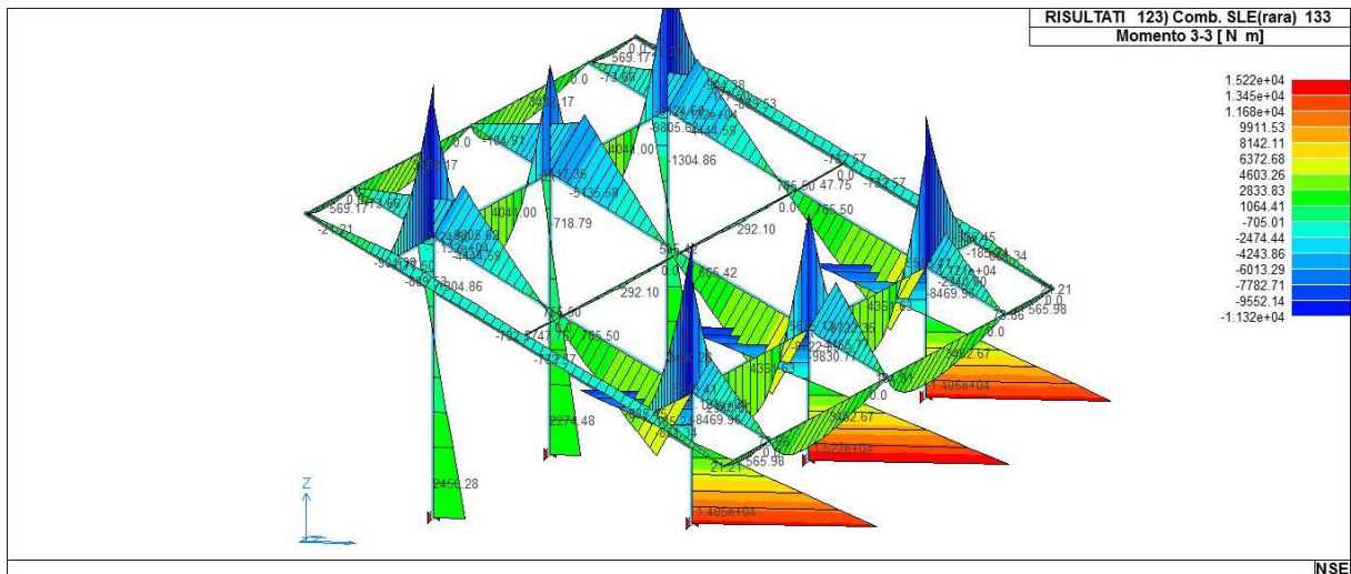
43_RIS_M3_123_Comb. SLE(rara) 133
