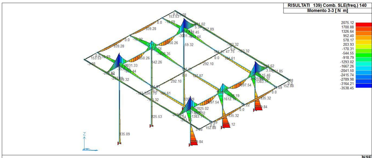
43_RIS_M3_139_Comb. SLE(freq.) 140
