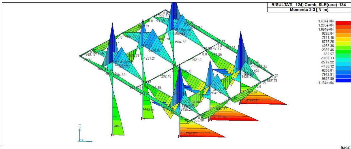
43_RIS_M3_124_Comb. SLE(rara) 134
