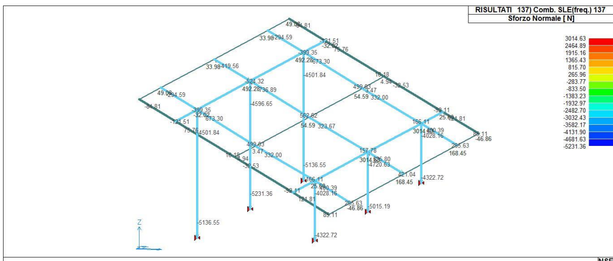
43_RIS_N_137_Comb. SLE(freq.) 137
