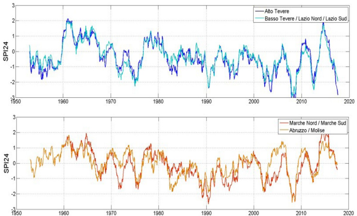
Figura 6 - Standardized Precipitation Indices a 24 mesi (SPI24)
