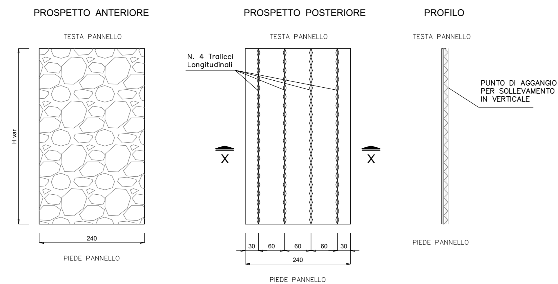
PANNELLI PREFABBRICATI IN C.A.V. scala 1:50 MISURE IN cm
