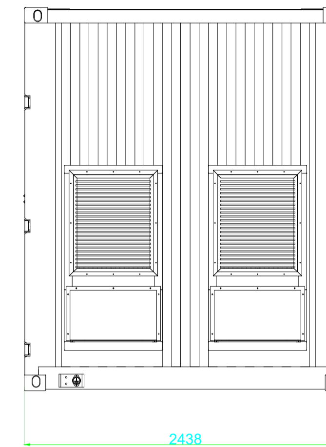
Left view
