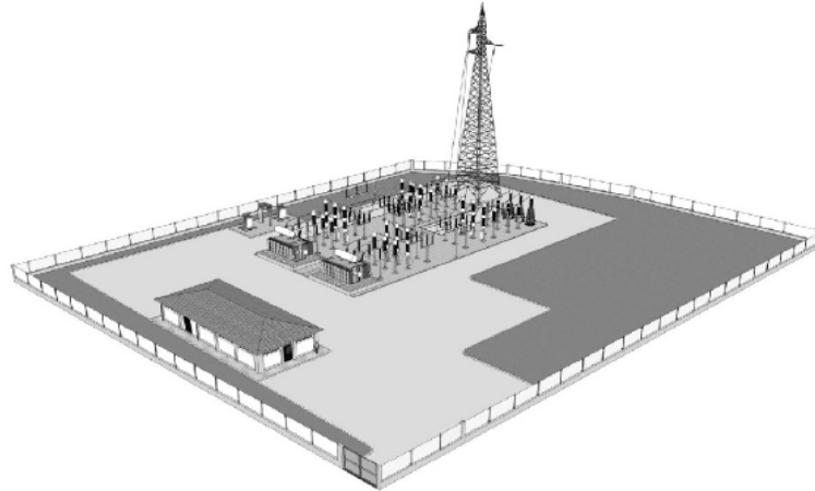
A16 - Cabina primaria isolata in aria (132/150-15/20 kV)
