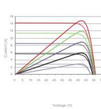
Current-Voltage & Power-Voltage Curves (665W)
