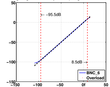
Level Linearity Test at 15.849Hz for Channel BNC_6 C-weighting Gain 0dB passed (Range: 98dB Tol.: 70dB)
