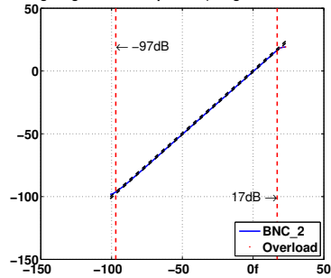
Level Linearity Test at 15.849Hz for Channel BNC_2 Z-weighting Gain 0dB passed (Range: 106dB Tol.: 70dB)
