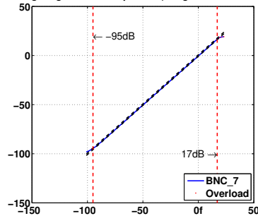
Level Linearity Test at 15.849Hz for Channel BNC_7 Z-weighting Gain 0dB passed (Range: 106dB Tol.: 70dB)
