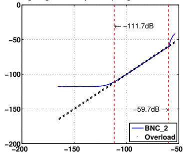
Level Linearity Test at 15.849Hz for Channel BNC_2 A-weighting Gain 0dB passed (Range: 52dB Tol.: 20dB)
