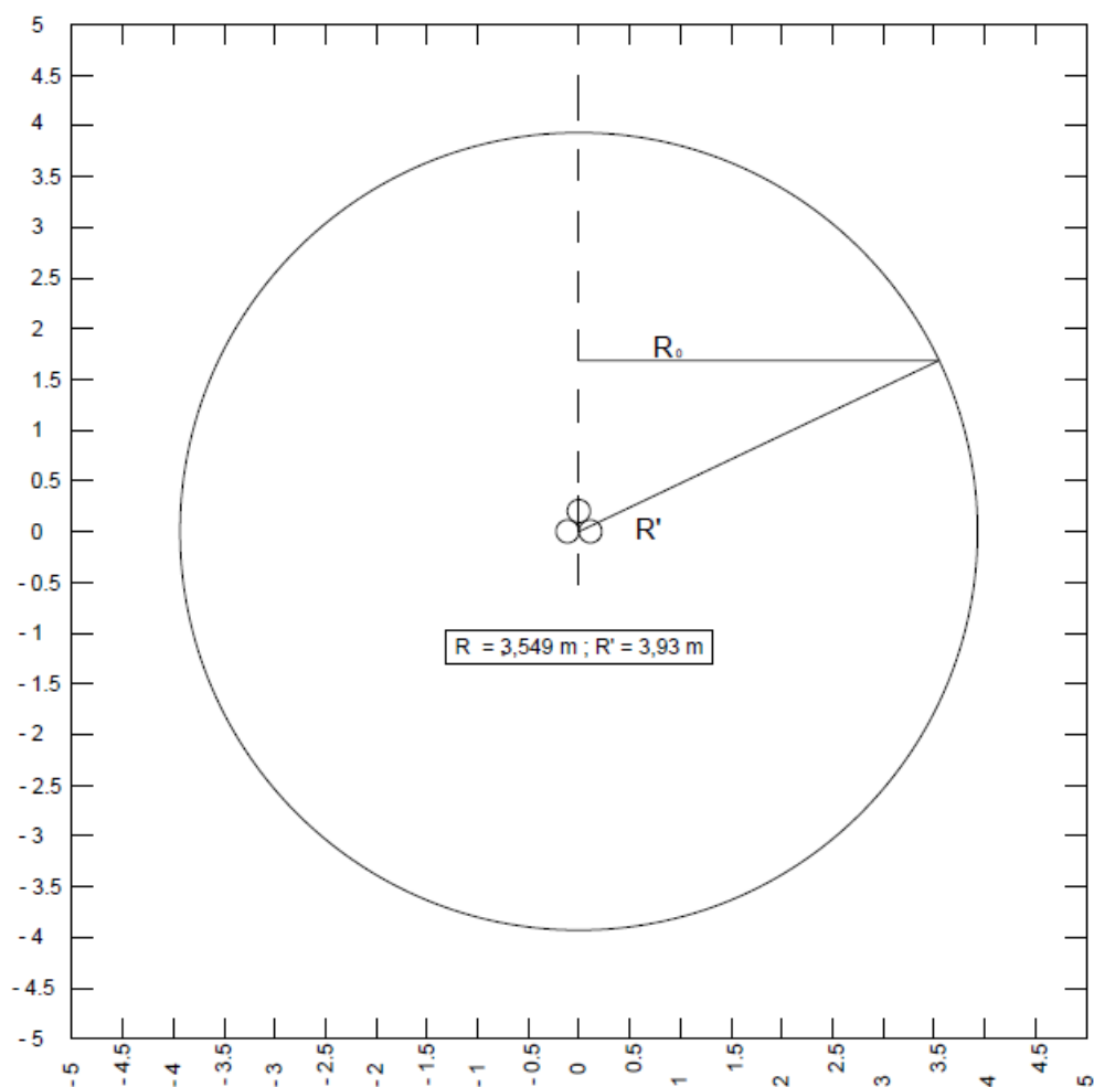
Cavi AT posati a trifoglio S = 0.20 \text{ m} ; I=944,40\text{A}
