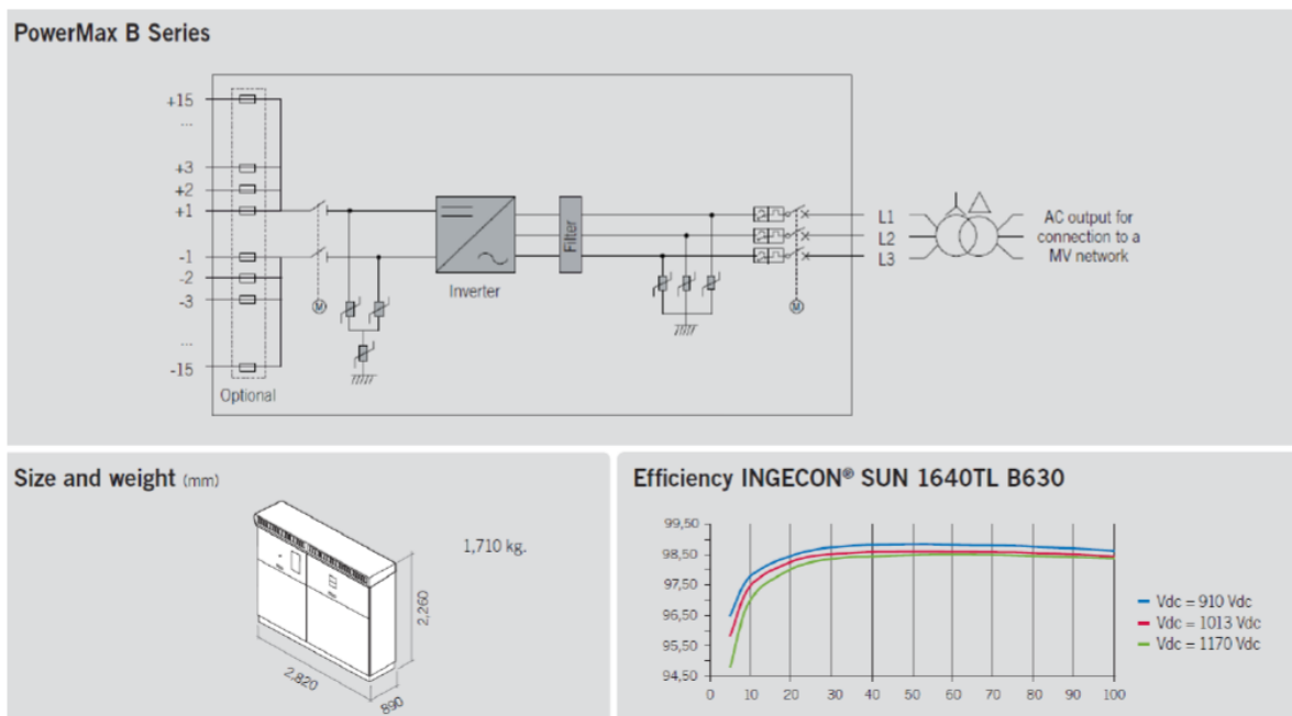
Datasheet inverter
