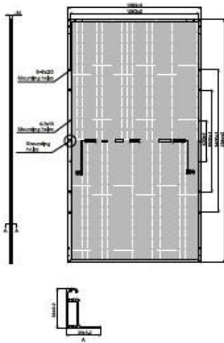
Dimensions of PV Module Unit: mm
