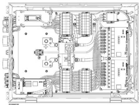
Combiner Box
