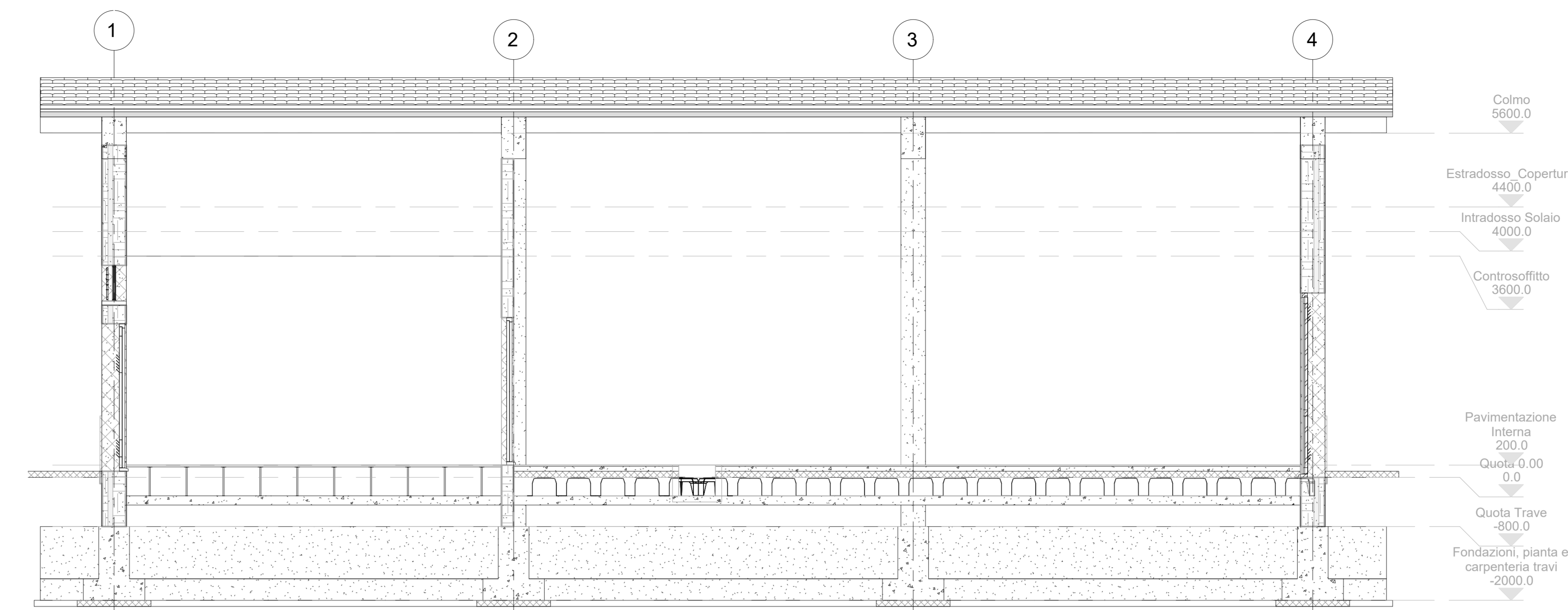
3 Arc.1 1:50
