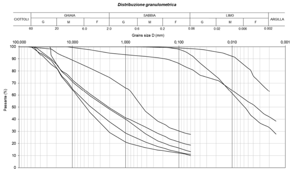
Figura 8-8 – Curve granulometriche
