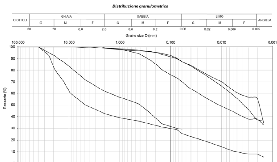
Figura 8-9 – Curve granulometriche
