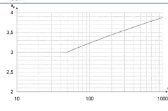
Figure B.2 - Peak factor k_p = \sqrt{2 \cdot \ln(v \cdot T)} + \frac{0,6}{\sqrt{2 \cdot \ln(v \cdot T)}} or k_p = 3 whichever is larger
