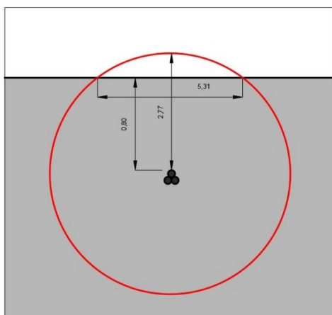
Cavi ARG7H1E(X) 18/30 kV 185 mm 2
