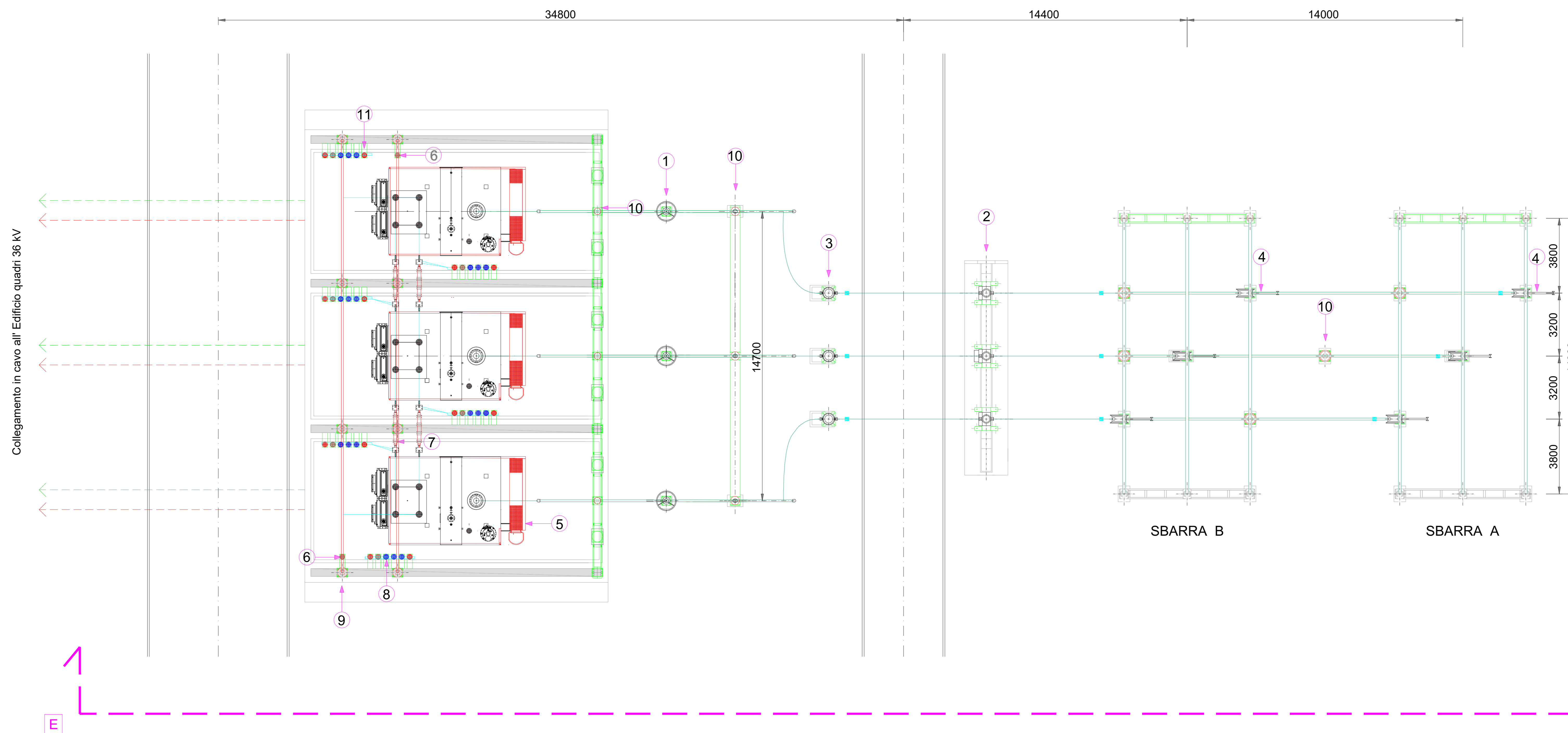
Stallo TR 220/36 kV da 250 MVA - Scala 1:100
