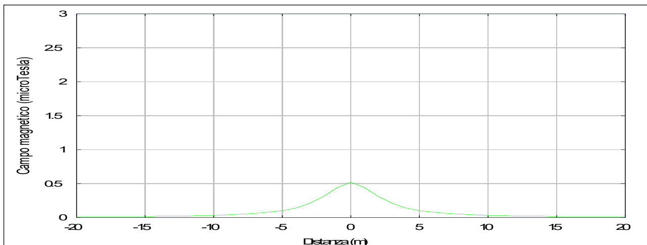
Figura 1: ELF In = 763A
