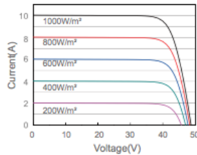
Current-Voltage Curve JAM72S01-380/PR
