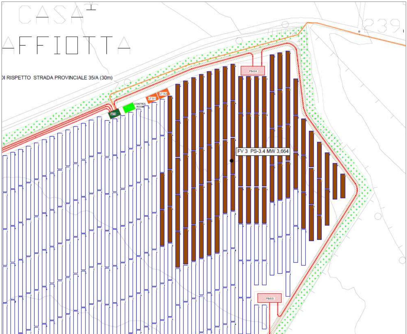
Planimetria campo PS-3.4
