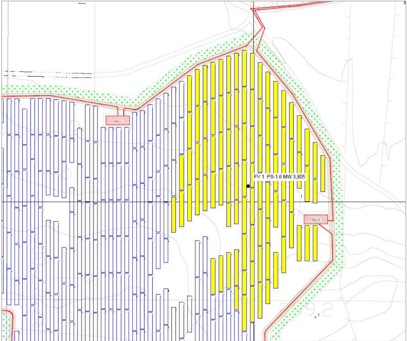
Planimetria campo PS-1.6
