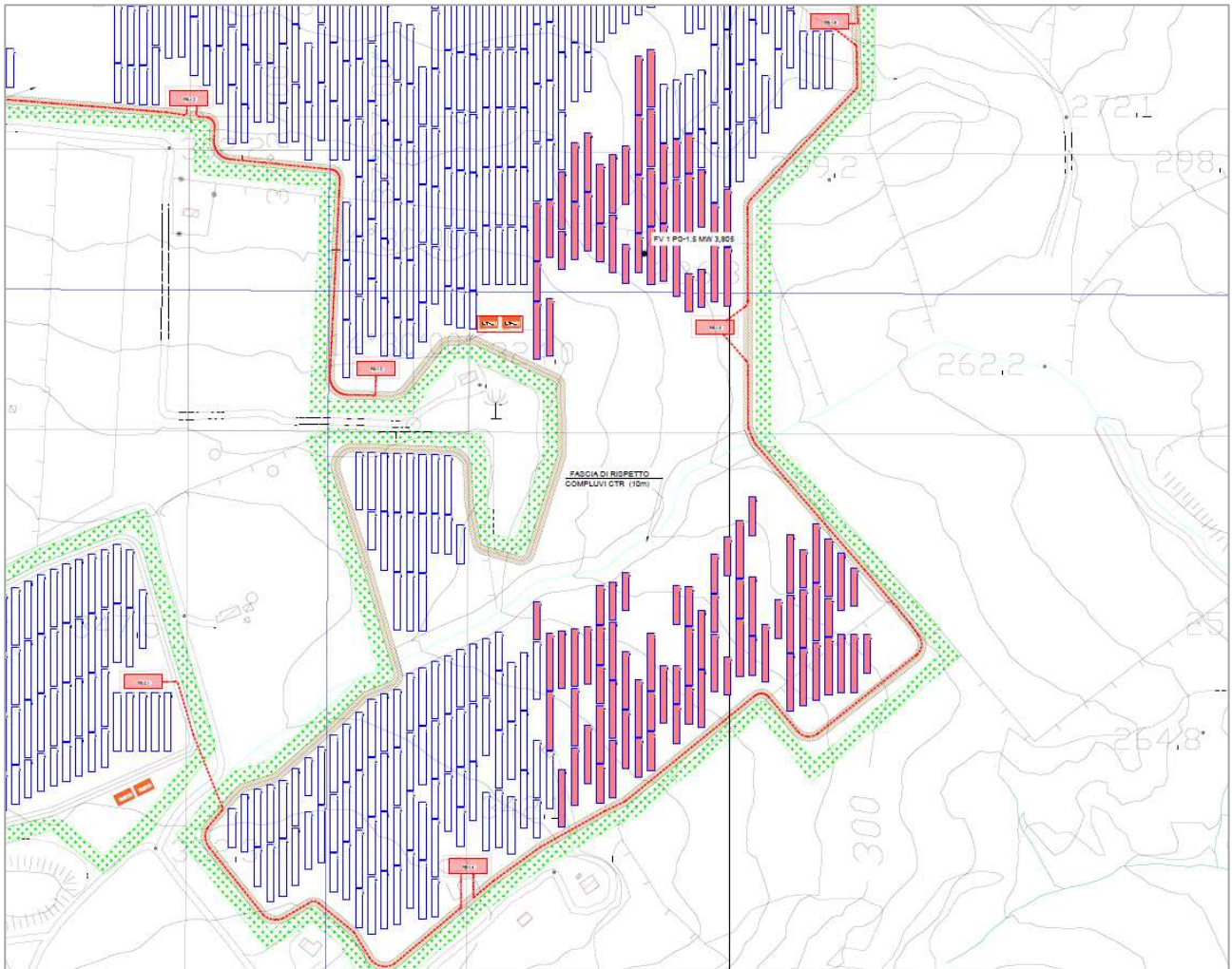
Planimetria campo PS-1.5
