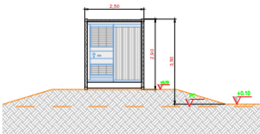
Figura 6.4: vista laterale Power station
